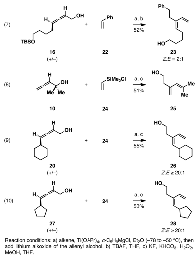
Figure 5. Reductive cross-coupling reactions of allenyl alcohols with styrene and chlorodimethylvinylsilane.
