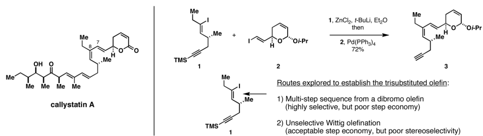
Figure 2. Difficulties experienced in establishing the C6-C9-( Z,E )-diene of callystatin A.
