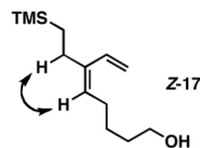
Figure 4. Exploring the basic bond construction: Reductive cross-coupling between substituted allenes and vinyltrimethylsilane.
