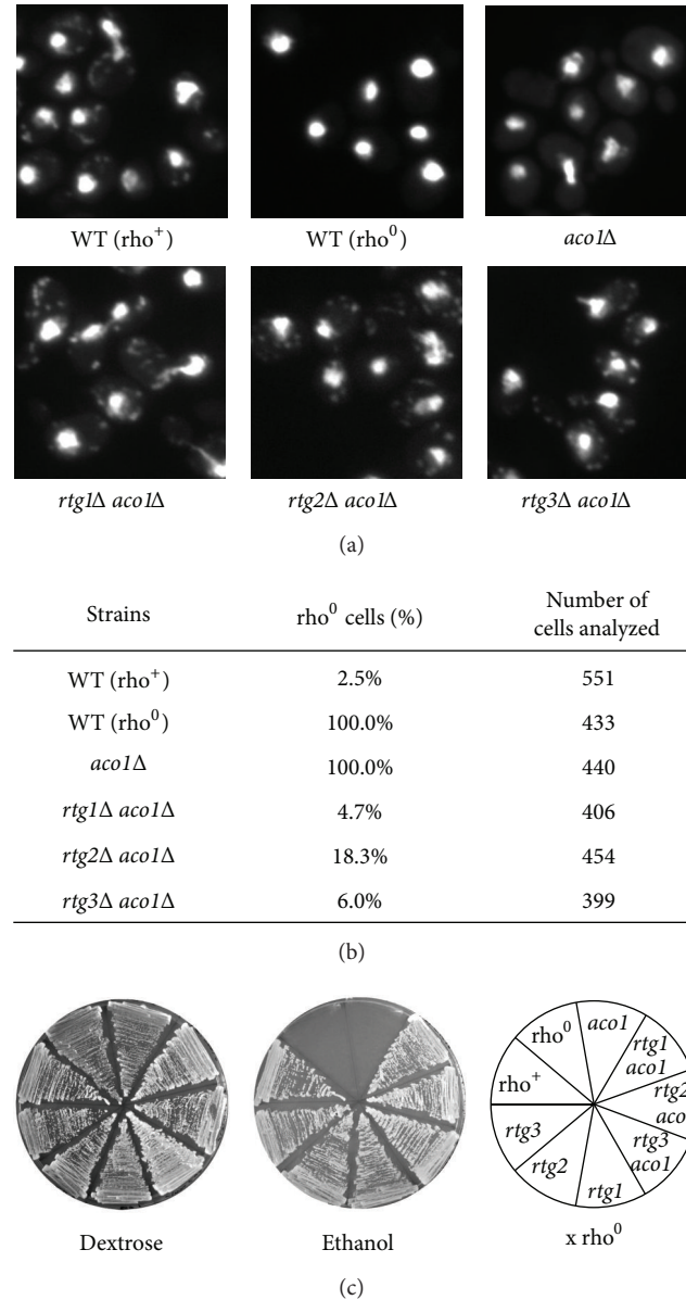
FIGURE 2: mtDNA is maintained in rtg1 \Delta aco1 \Delta , rtg2 \Delta aco1 \Delta , and rtg3 \Delta aco1 \Delta mutant cells. (a) Cells grown exponentially in YPD medium were stained with DAPI and then examined using fluorescence microscopy. WT ( \rho^+ ), BY4741; WT ( \rho^0 ), BY4741 \rho^0 ; aco1 \Delta , ZLY2630; rtg1 \Delta aco1 \Delta , ZLY2648; rtg2 \Delta aco1 \Delta , ZLY2631; rtg3 \Delta aco1 \Delta , ZLY2652. (b) Quantitative analysis of the percentage of \rho^0 cells in yeast strains based on DAPI-staining images. (c) mtDNA in rtg \Delta aco1 \Delta double mutant cells is functional. Strains as described in (a) as well as rtg1 \Delta , rtg2 \Delta , and rtg3 \Delta single mutants were crossed to a \rho^0 tester strain (X \rho^0 ) of opposite mating type. Diploids were selected and grown on YPD (Dextrose) and YPEthanol (Ethanol) medium. Pictures of cells were taken after 3 days' growth at 30°C.
