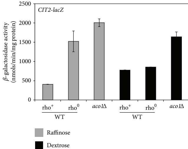
FIGURE 1: The RTG pathway is activated in aco1\Delta mutant cells grown in dextrose medium. Wild-type \rho^+ (WT, BY4741), its \rho^0 derivative, and aco1\Delta (ZLY2603) mutant strains were transformed with a centromeric plasmid encoding a CIT2-lacZ reporter gene (pCIT2-lacZ) and transformants were grown in YNBCasR (Raffinose) and YNBCasD (Dextrose) medium to mid-logarithmic phase. Cells were collected and \beta -galactosidase assays were conducted as described in Section 2.
