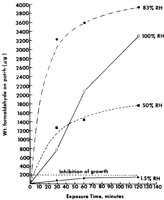
FIG. 2. Amount of formaldehyde from paraformaldehyde adsorbed on cotton patches (5/8 inch, ca. 1.59 cm). Vapor concentration is 10.6 mg/liter of air.
