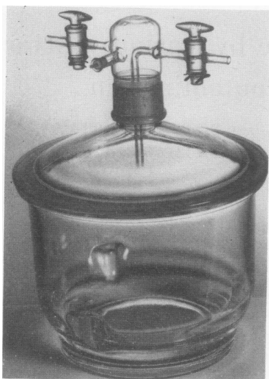
FIG. 1. Formaldehyde exposure chamber.
