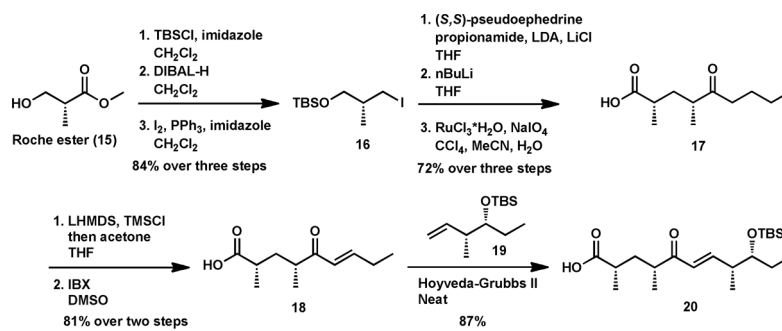
Scheme 2. Second generation 24 approach to Pik pentaketide.
