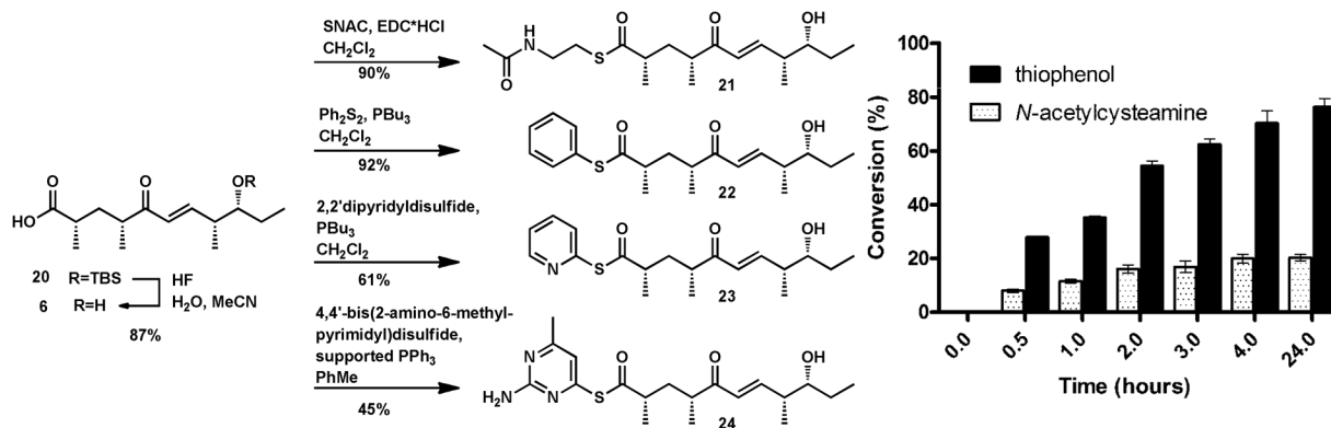
Figure 2. Synthesis and evaluation of activated Pik pentaketides. Enzymatic reaction conditions: 1mM Pik pentaketide, 10mM MM-NAC ( vide infra ), 0.5mM NADP + , 2.5mM glucose-6-phosphate, 0.5 unit/mL glucose-6-phosphate dehydrogenase, 8mM 2-vinylpyridine, and 1μM purified PikAIII-TE, 1–24 hours. Conversion of 21 and 22 to 10-deoxymethyonolide ( 7 ) was monitored (HPLC) with data represented as mean ± standard deviation. n=3
