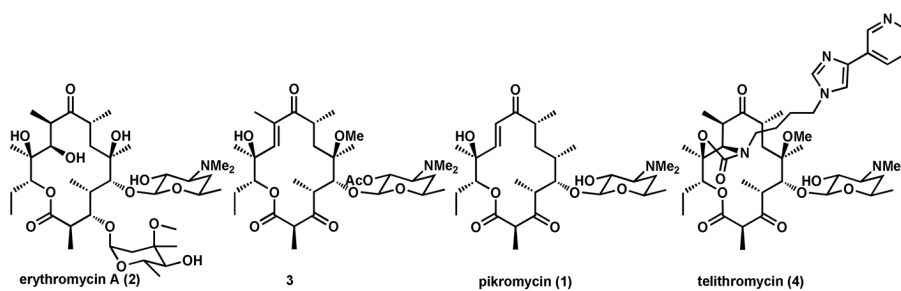
Figure 1. Macrolide antibiotics including ketolide 3 , 60 an intermediate en route to telithromycin, from erythromycin A.
