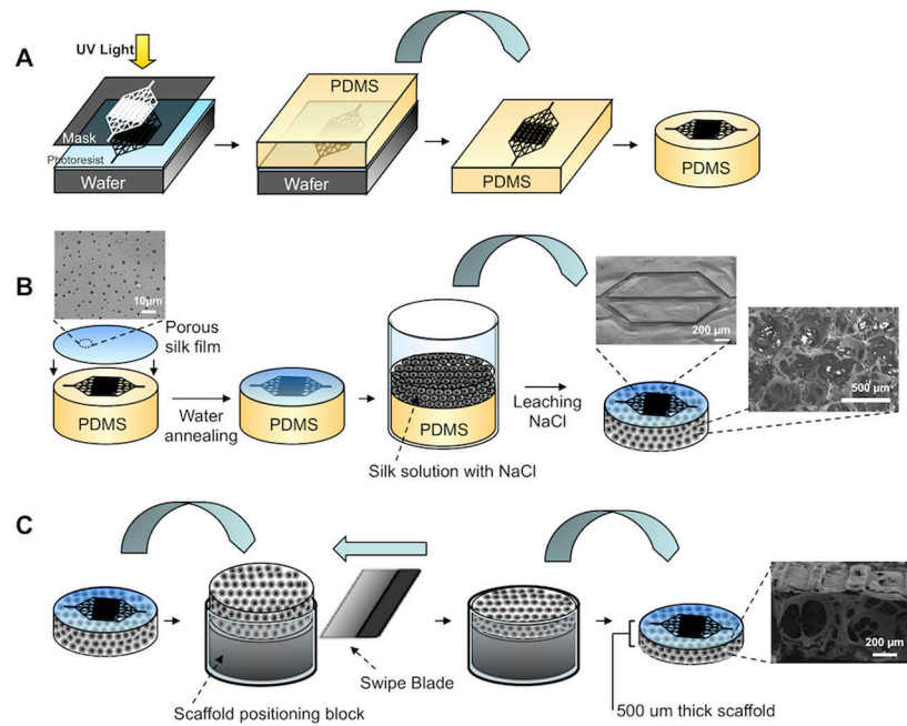
Figure 1. Schematic of micropatterned porous silk scaffold fabrication. (A) Microfluidic channel patterns are transferred from a silicon wafer to polydimethyl siloxane (PDMS) using standard photolithography and soft lithography techniques. The PDMS mold is trimmed to the desired shape and size. (B) A porous silk film is cast over the PDMS mold and water annealed to induce \beta -sheet crystallinity. An aqueous-derived salt leached silk scaffold is assembled over the silk film. The scaffold is cured and removed from the PDMS mold. SEM images show patent microchannels on the surface of the scaffold and 100–350 \mu\text{m} diameter interconnected pores in the bulk of the scaffold. (C) The scaffold thickness is trimmed by swiping a blade across the top of a positioning mold, which removes the bit of exposed scaffold. This mold allows for tunable control over the resulting thickness of the scaffold by changing the height of the positioning block.
