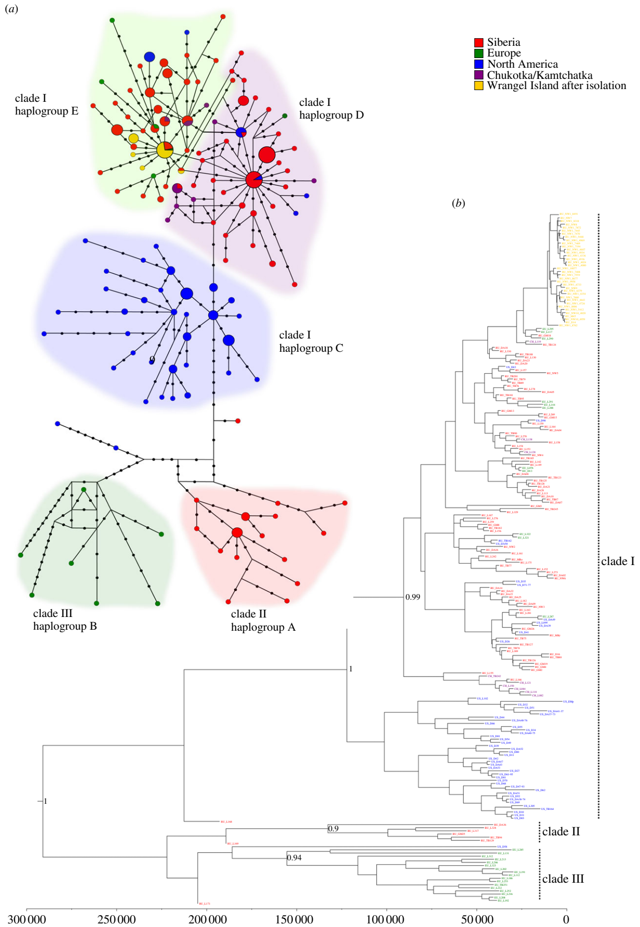
Figure 1. Median-joining haplotype network and Bayesian phylogeny of woolly mammoth mtDNA sequences. (a) Haplotype colours indicate their geographical location. Shaded areas correspond to haplogroups as in Debruyne et al. [11]. Black dots represent missing haplotypes. Haplotype size is proportional to its frequency within the dataset except for the three most frequent haplotypes within haplogroups D and E that have frequencies above 10. (b) The labels at the tips of the phylogeny are coloured according to the geographical origin of the sequences. The timescale on the x -axis is in calendar years before present. Bayesian posterior probabilities of major internal nodes above 0.8 are shown.
