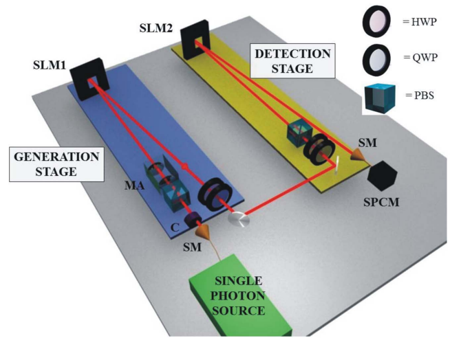
Figure 2 | Sketch of experimental setup for generating and testing photonic MUBs in dimension six. The polarization state is controlled by suitable sequences of wave plates, while the OAM mode is controlled by SLMs and single-mode fibers. Legend: SM - single-mode fiber; C - polarization compensation waveplates; HWP - half-wave plate; QWP - quarter-wave plate; MA - radial mode adjustment lens set; SLM - spatial light modulator; SPCM - single-photon counter module; PBS - Polarizing Beam Splitter.
