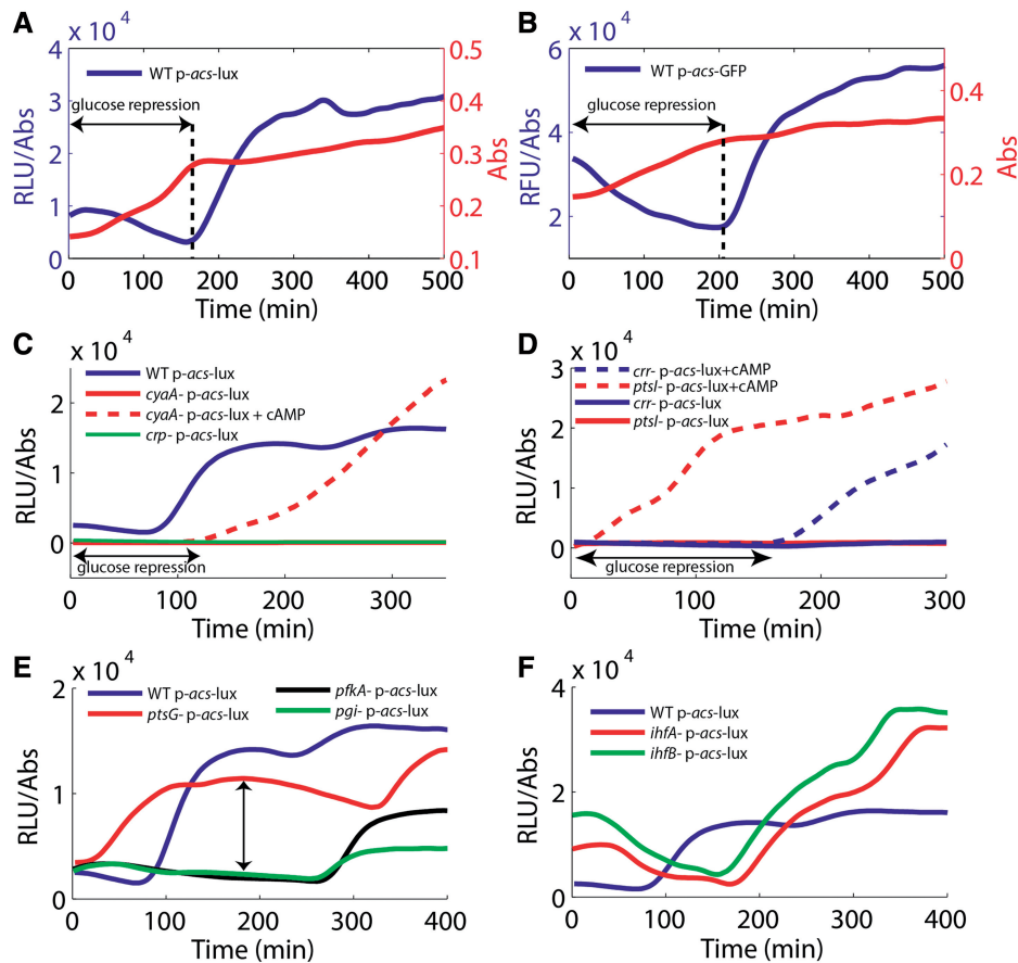
Figure 4. Dynamics of gene expression of known mutants in liquid minimal medium containing glucose and acetate: (A) The expression profile of the acs luciferase reporter plasmid shows that acs expression is induced when glucose is exhausted. (B) The acs expression profile using GFP as a reporter is identical to the profile observed with luciferase (A). (C) acs expression is completely absent in crp and cyaA strains. cAMP added to the medium (5 mM) at the beginning of the experiment complements the cyaA strain but glucose repression is maintained. (D) Low expression of acs in the crr and ptsI strains. cAMP added to the medium at the beginning of the experiment directly complements the ptsI strain during growth on glucose, whereas the crr strain only responds once glucose is exhausted. (E) In the ptsG mutant, acs induction is delayed because glucose is consumed more slowly. Moreover, acs expression during glucose consumption is much stronger than in the WT strain. The glycolysis mutants pgi and pfkA also grow more slowly, but acs expression remains low in exponential phase. (F) The expression profiles of the ihfA and ihfB strains show stronger acs expression than the WT during growth on acetate. The highly similar expression kinetics of the two mutants (with genes located at different sites on the chromosome) shows the high internal consistency of the method.
