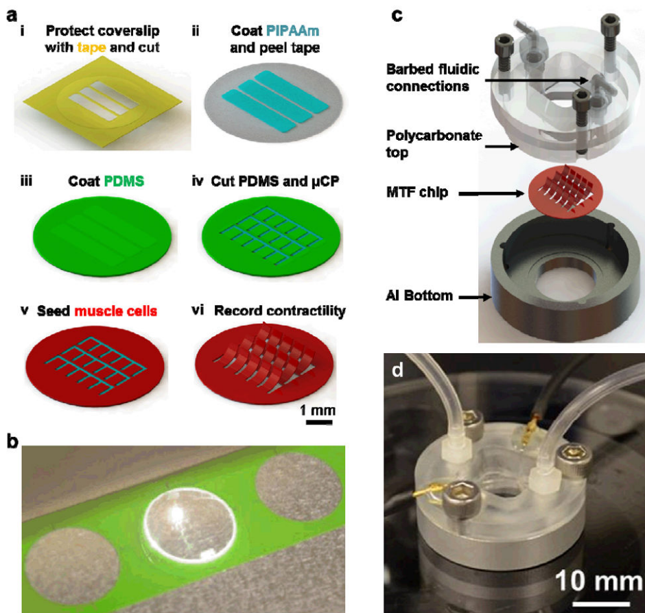
Figure 1. Higher throughput heart on a chip and fluidic microdevice. (a) A schematic of fabrication process (i) A glass coverslip is covered with protective tape and PIPAAm islands are cut into by an engraving laser and peeled using a sharp tweezer. (ii) A thin layer of PIPAAm is spun coat, (iii) the tape is removed and PDMS is spun coat. (iv) The boundaries of thin films are then cut into the PDMS and peeled. (v) The chip is then ready for micro contact printing of fibronectin and cell seeding. (vi) Upon PIPAAm dissolution, individual MTFs are released from the surface and interrogated optically. (b) Image of the engraving laser processing MTFs in an 18 mm diameter chip. A batch of multiple chips can be fabricated by this computer aided design process. (c) Exploded view of the conception and assembly of a fluidic device which fits an 18 mm chip. The device consists of an aluminum bottom with a recess to hold the chip, a transparent polycarbonate top held in place by three screws and barbed fittings for fluidic input and output. (d) Image of an actual device in action. The connection for electrical field stimulator can also be seen in addition to the fluidic tubing.
