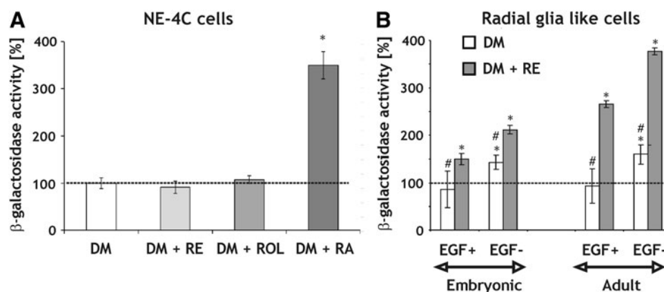
FIG. 3. Retinoid production by NE-4C neural stem cells and RGI cells assayed by measuring \beta -galactosidase activity in F9 RA-reporter cells. (A) NE-4C cells were kept either in DM or treated with 1 \mu M RE, ROL or RA for 48 h (DIV0-2), then washed thoroughly and kept in retinoid-free medium for 6 more days (DIV2-8). The RA-reporter cell assay was carried out on DIV8 incubating the differentiated NE-4C cells in cocultures with the reporter cells. The method allowed direct, cell to cell activation of the transgene. * P < 0.01 . (B) \beta -galactosidase response of F9 RA-reporter cells to conditioned media obtained either from nondifferentiated (EGF+) or differentiated (EGF-) embryonic or adult RGI cells grown in the absence (DM) or presence (DM + RE) of retinyl acetate for at least 2 weeks before, as well as during the assay. The optical density (OD) values of the assays (A, B) were related to the \beta -galactosidase activity (100%; indicated by the dashed line) of control F9 cells. * P < 0.01 ; significant difference from F9 cells; # P < 0.05 ; significant difference from cells grown in DM + RE.
