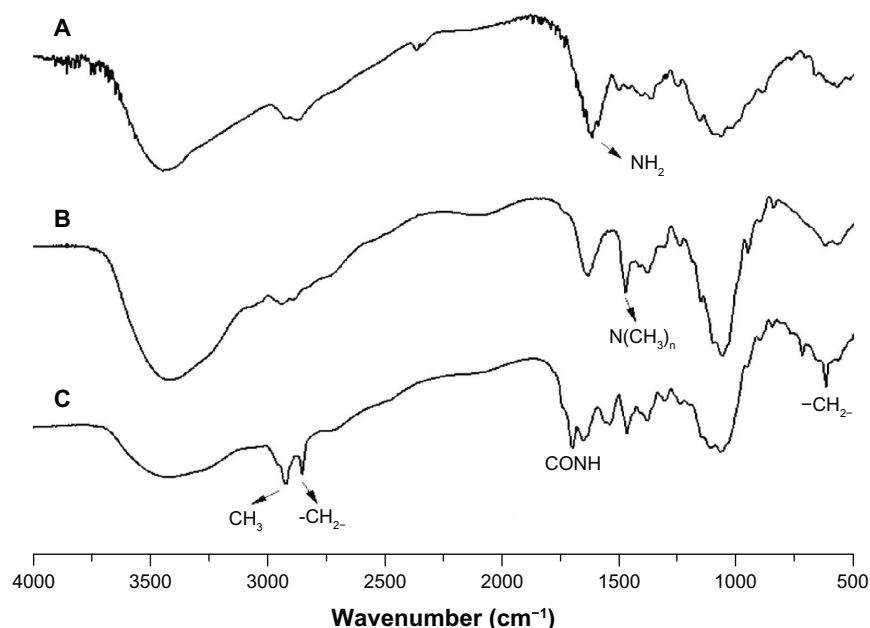
Figure 2 FTIR spectra of chitosan (A), TMC2 (B), and CA-TMC2 (C).
