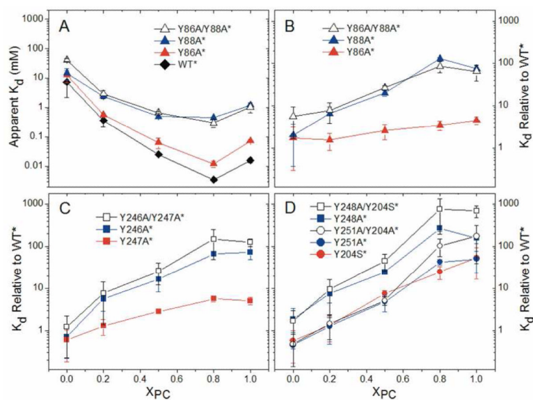
FIGURE 5. Binding of PI-PLC Tyr variants to SUVs. Apparent K_d (A) and apparent K_d relative to WT* (B, C, and D) as a function of X_{PC} . The error bars are the largest uncertainties generated during the FCS data analysis, either the standard deviations from two independent repeats or the uncertainty generated by error propagation for the two independent data sets.
