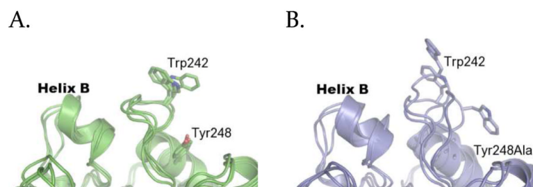
FIGURE 4. Effect of the Y248A mutation on PI-PLC. Structure of the interfacial binding sites of WT PI-PLC (A) and Y248A (B) after 20 ns MD simulations in water, from three independent simulations in each case.
