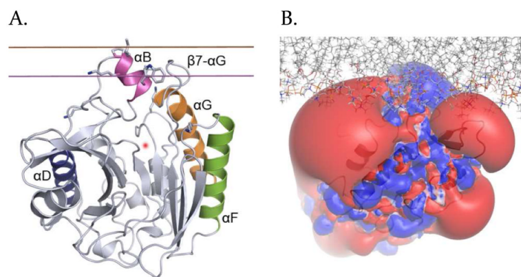
FIGURE 1. PI-PLC membrane binding orientations from MD simulations. A. IMM1 orientation of PI-PLC used to initiate the simulations with explicit lipids. Helices B, D, F and G are magenta, blue, green and orange, respectively. The active site is represented by a red fuzzy dot. B. Positioning of PI-PLC in the explicit bilayer model. Lipids are represented with thin sticks colored according to the atomic elements (N: blue, O: red, P: orange, C and H: grey). Electrostatic potential of PI-PLC; the equipotential contours at -/+ 1\text{kT} (red/blue) calculated using APBS. 25 The potential between -1\text{kT} and +1\text{kT} is mapped on the molecular surface (negative: red, positive: blue).
