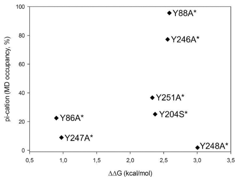
FIGURE 6. Comparison between occupancies of predicted cation-π interactions from the simulation and evaluation of \Delta\Delta G (kcal/mol) from FCS measurements for PI-PLC WT* and single tyrosine mutants.
