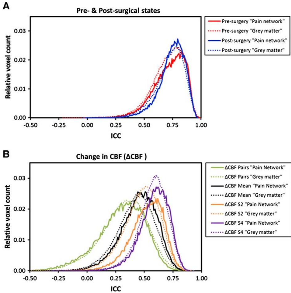
Fig. 5. ICC distributions of the pre- and post-surgical states (A) together with the ΔCBF (change in CBF) (B). Plots show the relative number of activated voxels against ICC score for the grey-matter (dotted lines) and activated pain network (solid lines).
