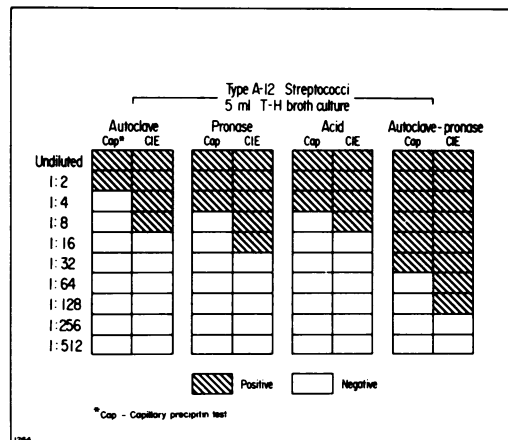
FIG. 4. Comparison of the efficiency of four methods of extracting group-specific polysaccharide. Also demonstrated is the increased sensitivity of the CIE method of grouping streptococci over the capillary precipitin tube test.
