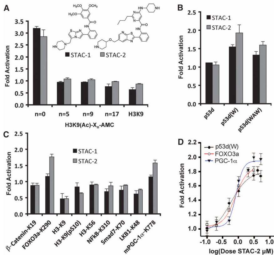
Fig. 1. SIRT1 activation by STACs on native peptide sequences. (A) SIRT1 activation by 50 \mu M STAC-1 or 5 \mu M STAC-2 with peptides bearing an AMC moiety at the indicated positions, where X n represents the number of amino acids between the acetylated lysine and the AMC. (B) SIRT1 activation by STACs on hydrophobic patch peptides. Complete amino acid sequences of peptides bearing tryptophan (W) or tryptophan and alanine substitutions (WAW) are provided in the supplementary materials. (C) SIRT1 activation on native peptide sequences of known targets (detailed in the supplementary materials). (D) Dose-response curves for STAC-2 as measured by PNC1-OPT assay; data are means \pm SEM ( n = 3 ).
