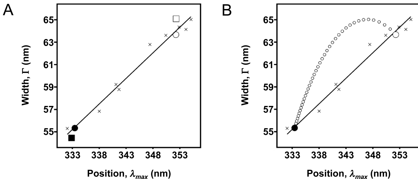
Fig. 4. Position-width analysis of tryptophan fluorescence from folded and unfolded outer membrane proteins. Positions ( \lambda_{max} ) and widths ( \Gamma ) come from fits to Eq. (3). The solid line is a linear fit to data from spectra of N -acetyl-tryptophan-amide dissolved in different solvents or mixtures of solvents (crosses). (A) Two proteins, FadL (filled square) and OmpW (filled circle), were folded into LUVs of DLPC in 1.5 M guanidine HCl. The two proteins were also unfolded in the presence of the same LUVs but in 5.5 M guanidine HCl (open symbols of the same shapes). (B) Simulated data (small open circles) showing the expected heterogeneity of tryptophan environments when different fractions of an ensemble of OmpW molecules are folded versus unfolded. These different fractions could be obtained, for example, when a sample of OmpW is titrated into different concentrations of guanidine HCl. Each data point along the arc comes from Eq. (12) and represents a 2.5% step in a mixture of the folded and unfolded states. The endpoints of the arc (large circles) were taken from the actual data for OmpW shown in (A).
