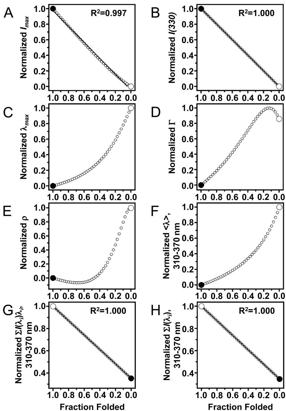
Fig. 6. Not every spectral parameter of tryptophan fluorescence linearly depends on fraction folded. The endpoints of each plot (large circles) were taken from actual data for folded and unfolded samples of OmpW with LUVs of DLPC in 1.5 M and 5.5 M guanidine HCl, respectively. Other data points (small circles) come from Eq. (12) and represent 2.5% steps of simulated mixtures of the folded and unfolded samples. (A) Peak intensity ( I_{max} ). Solid line represents a linear fit to the data points. (B) Emission intensity at 330 nm. Solid line represents a linear fit to the data points. (C) Position of maximum emission ( \lambda_{max} ). (D) Spectral width ( \Gamma ) at half the peak intensity. (E) Log-normal asymmetry parameter ( \rho ). (F) Average emission wavelength \langle \lambda \rangle using a window of emission from 310–370 nm. (G)
