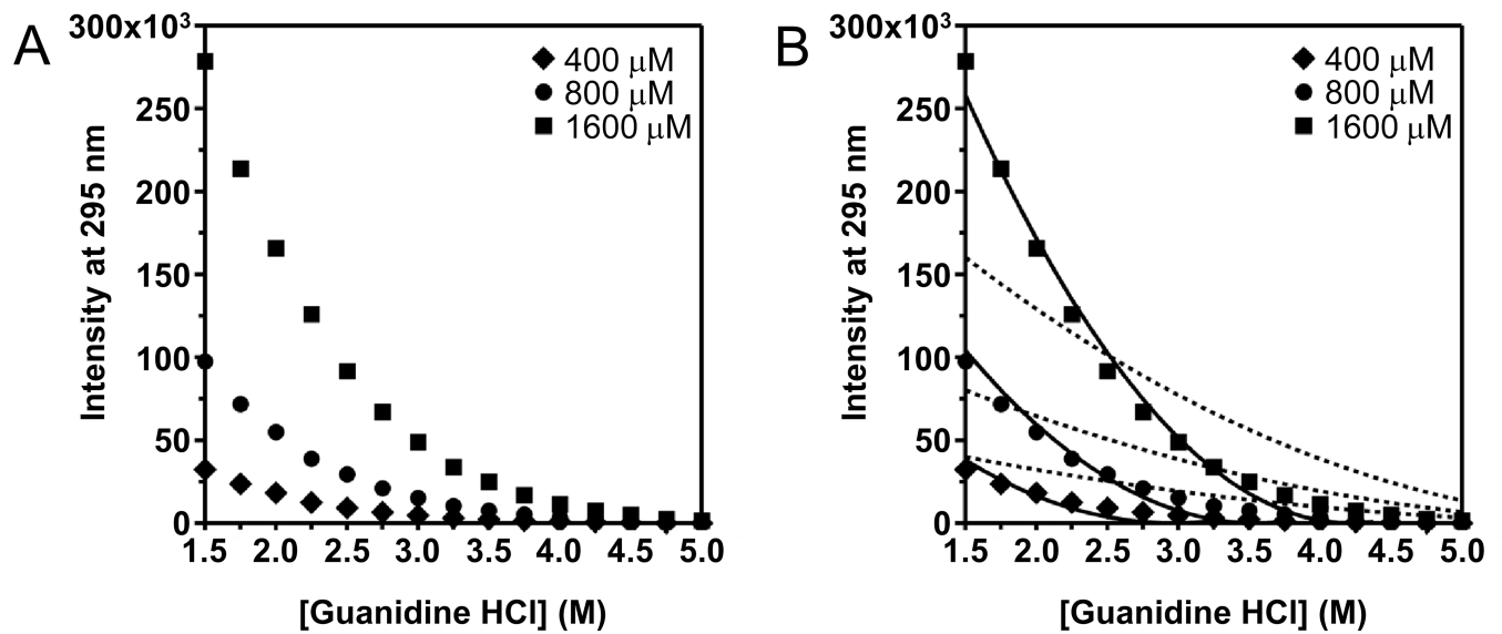
Fig. 3. Denaturants can reduce light scattering from LUVs by matching the refractive index of the lipid bilayers. Peak intensities of RGD light scattering by LUVs of DLPC at an excitation wavelength of 295 nm are plotted. Dotted lines represent fits to Eq. (9). Solid lines represent fits to Eq. (11). The background buffer for all samples was 2mM EDTA and 100 mM citrate, pH 3.8. (A) Effect of the number of LUVs on their light scattering at different concentrations of the solute guanidine HCl. (B) Effect of the solute sucrose on the light scattering at a lipid concentration of 800 \mu\text{M} .
