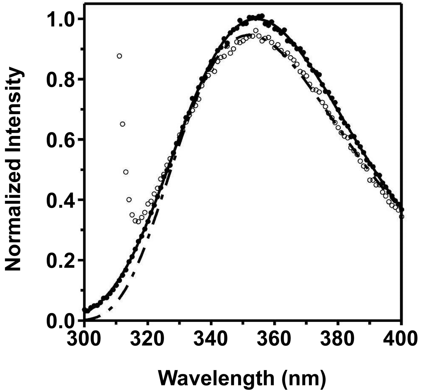
Fig. 2. Light scattering changes the spectral properties of tryptophan fluorescence. Two samples of L-tryptophan zwitterion were dissolved at a concentration of 6.0 \mu\text{M} in a background buffer of 2\text{mM} EDTA, and 100\text{mM} citrate, pH 3.8. One sample included LUVs of DLPC (open circles) at a lipid concentration of 800 \mu\text{M} . The solid line represents a fit of Eq. (1) to the open circles. The other sample had no LUVs (filled circles). The dot/dashed line represents the log normal distribution component of Eq. (3) fit to the filled circles.
