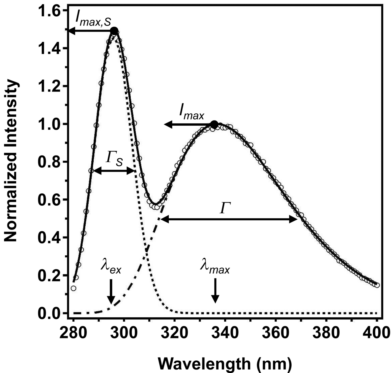
Fig. 1. Relative contributions of light scattering and tryptophan fluorescence emission to the observed data from a typical fluorescence experiment. The observed data (open circles) came from a sample of 400 nM FadL folded into LUVs of DLPC at a lipid-to-protein ratio of 2000-1 and in 1.5 M guanidine HCl, 2mM EDTA, and 100mM citrate, pH 3.8. The sample was excited at 295 nm, the excitation polarizer was set at 90°, and the emission polarizer was set at 0°. The sample pathlength was 10 mm, the excitation slits were 2.4 mm wide, and the emission slits were 2.0 mm wide. The solid line represents a fit to the observed data by a sum of a normal distribution and a log normal distribution as described by Eq. (3). Fit parameters from Eq. (3) are labeled next to the parts of the data that they describe. The dotted line is the normal distribution component of Eq. (2), which represents
