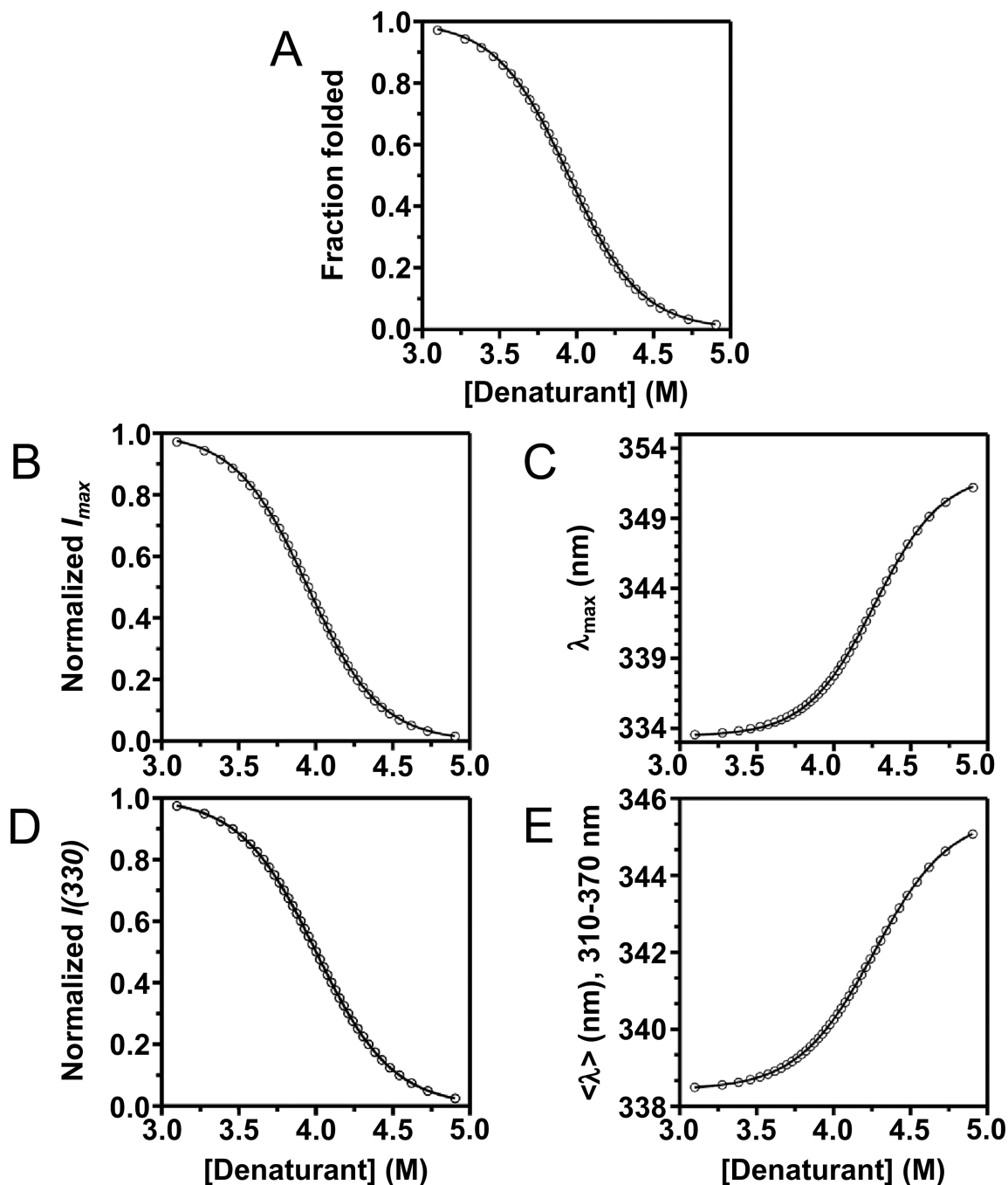
Fig. 7. Relationship of spectral parameters of tryptophan fluorescence to isotherms from chemical denaturation. The vertical-axis positions of the data points in each plot come from Eq. (12) and represent 2.5% steps of simulated mixtures of folded and unfolded samples of OmpW. The horizontal-axis positions of the data points come from Eq. (14) and represent a simulated equilibrium, two-state denaturant titration of OmpW at 37° C. For the simulation, \Delta G_w^o was assumed to be 10 kcal mol -1 , the m -value was assumed to be 5 kcal mol -1 M -1 , and the baseline regions were assumed to have zero slope. Solid lines represent a best fit of Eq. (14) to the simulated data. (A) Fraction folded. (B) Peak intensity ( I_{max} ). (C) Position of
