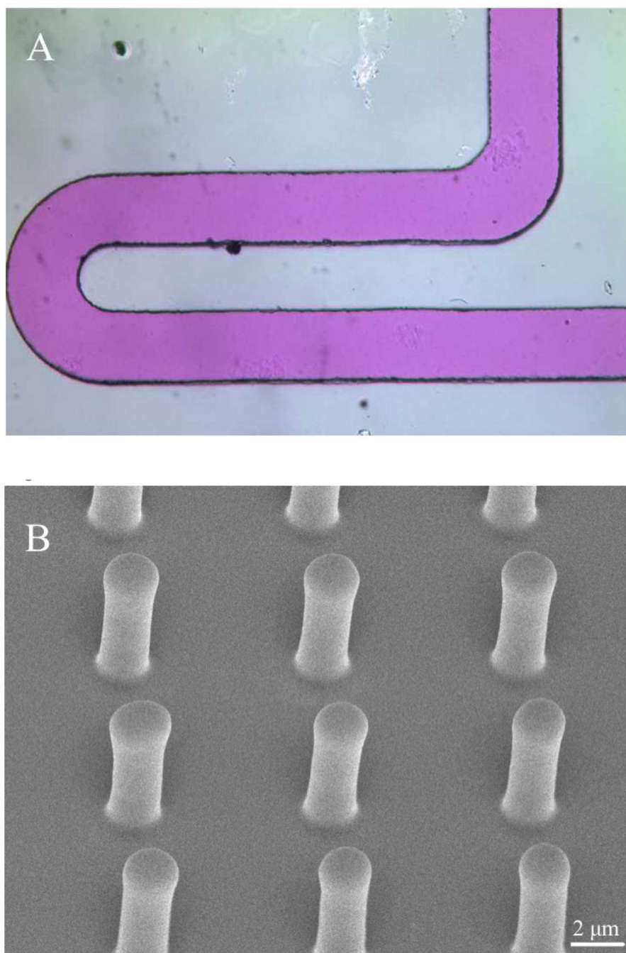
Fig 1. Image A shows 50 μm wide microchannel filled with dye. Image B shows an SEM image of 8 \times 2 μm (height x diameter) microposts with 7 μm spacing at 40° tilt molded in SEBS42, demonstrating the high fidelity replication.
