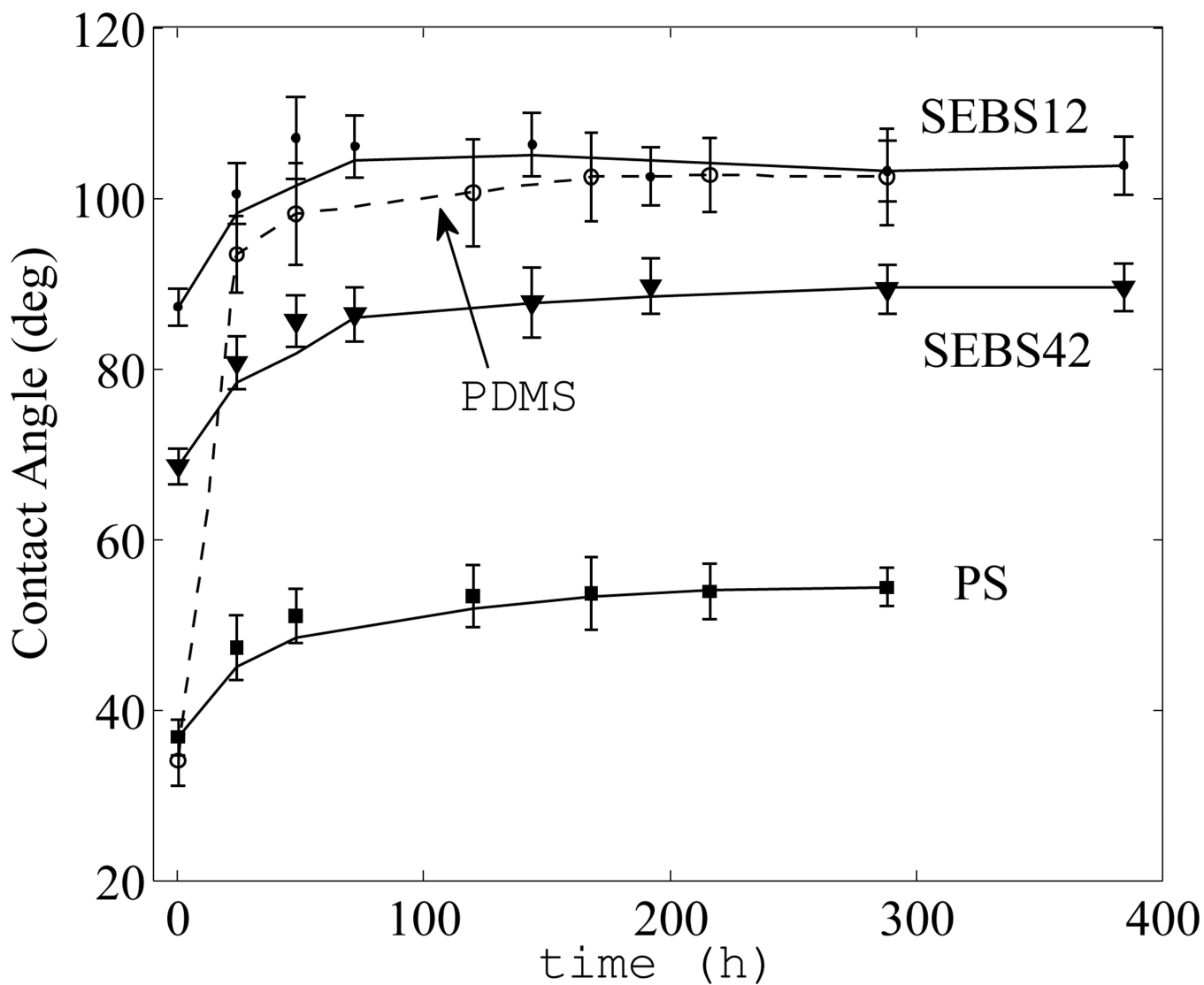
Fig 2. Advancing contact angle measurements following oxygen plasma treatment. SEBS42 (closed triangles) has greater wettability than SEBS12 (closed circles) and exhibits a moderate hydrophobic recovery. PS (closed squares) and PDMS (open circles, dashed line) are shown for reference. The recovery of SEBS is similar to PS and mild compared to PDMS. Error bars indicate \pm one standard deviation.
