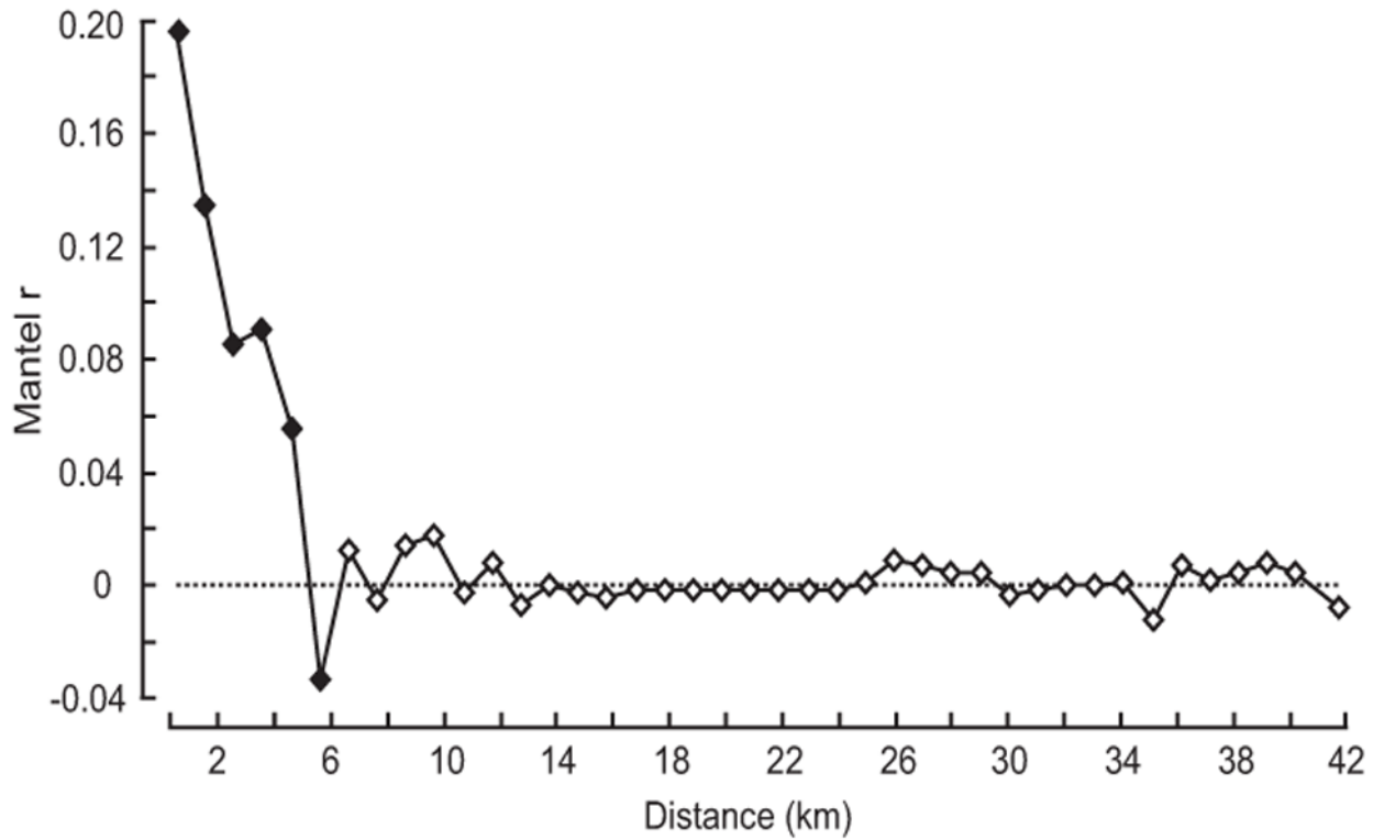
FIG. 4. Spatial autocorrelation of genetic distance and geographic distance. There is significant spatial autocorrelation at distances less than 5 km. The spatial autocorrelation rapidly dissipates with distance and is not significant at distances greater than 5 km.
