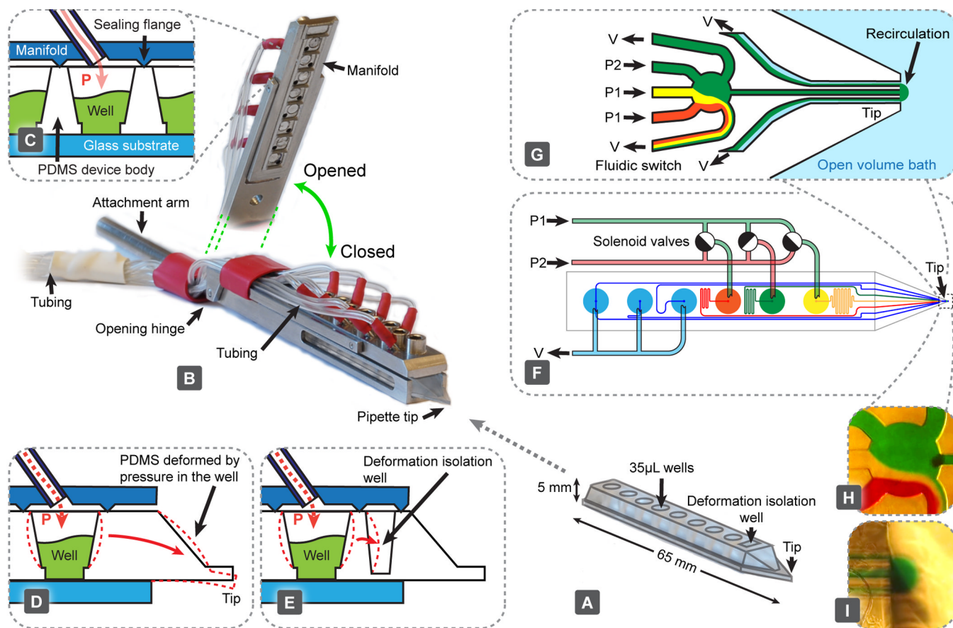
Fig. 1. The multifunctional pipette: components, construction and setup. (A) The PDMS microfluidic pipette tip. (B) The holder, shown in a closed state holding the tip. An elevated angle is also displayed to highlight the manifold's interfacing structure, which contacts the tip. (C) Pneumatic interface between the holder and the tip is formed with sharp flanges protruding from the manifold, which are pushed into the PDMS surrounding the well. Each well has an individual connection, through which pressure can be controlled. (D) Deformation associated with pressure change within the well. (E) Implemented solution to (D), minimising the effects through the use of an isolation well. Exemplary circuitry of a fast 3-solution switch, showing the driving mechanism (F) and the microfluidic switching junction near the tip (G). Microscopy images of a fluidic switching junction (H) and a recirculation volume (I) loaded with coloured water.
