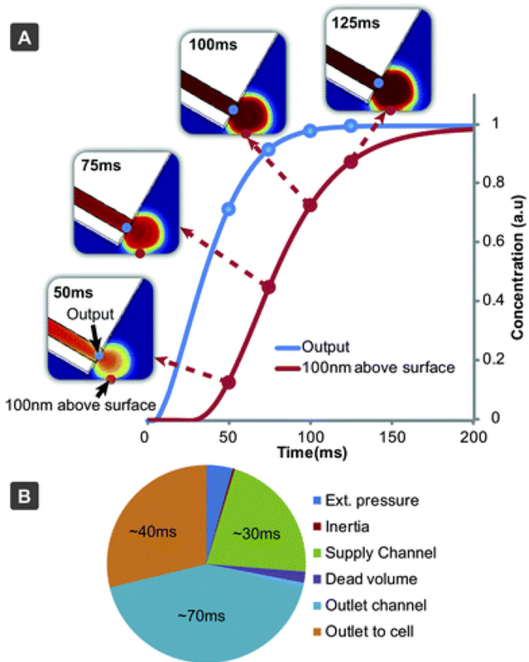
Fig. 3. Results of a computer simulation to model the fluidic exchange times close to the sample surface. (A) Concentration rise time near the surface (100 nm above) and at the channel output. (B) Contributing factors and influence to the solution exchange time, based on experimental results, simulations and calculations.
