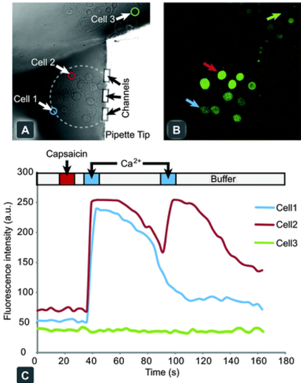
Fig. 4. Chemical stimulation and response of individual hTRPV1 expressing CHO cells, through activation with capsaicin. (A) Bright field microscopy image of adherent cell culture of hTRPV1 expressing CHO cells, with the pipette tip targeting a small collective. (B) Confocal fluorescent micrograph of Calcium Green™ loaded cells after stimulation with capsaicin and subsequent exposure to Ringer's solution, spiked with 10 mM calcium chloride. (C) A graph of individual cellular responses to the application protocol, with the delivery times highlighted above. Cells 1 and 2 are within the recirculation zone and display a positive activation response. Cell 3 is a representative cell from the background outside of the stimulation zone.
