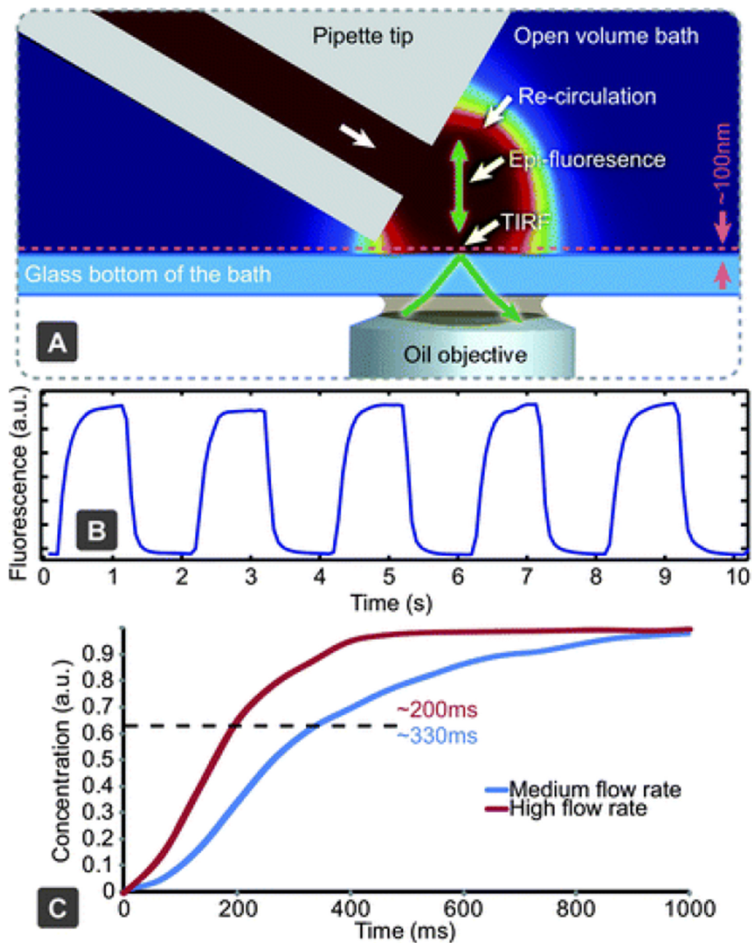
Fig. 2. Characterising solution exchange times. (A) Experimental setup using TIRF microscopy, to monitor solution exchange dynamics near the sample surface. The same setup can be used for epifluorescent measurements of a deeper region, through modification of the excitation angle. (B) Fluorescent intensity measurements of periodic solution exchange near a glass surface using TIRF. (C) Concentration rise time near the surface with high and medium flow rates ( \sim 10 and \sim 5 \text{ nL s}^{-1} , respectively).
