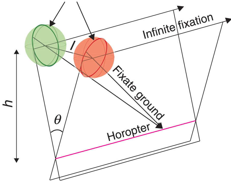
Figure 2. Vertical horopter and the ground. Green and red spheres represent the left and right eyes, respectively. The green and red circles represent the sheared empirical meridians associated with empirical corresponding points. When the eyes are fixated parallel to the ground at infinity, the vertical horopter is a horizontal line extending to meet fixation at infinity. For a given eye height and inter-ocular distance, the optimal shear angle places the horopter in the ground plane. Due to Listing’s Law, the horopter remains in the ground when the eyes fixate the ground in the sagittal plane.
