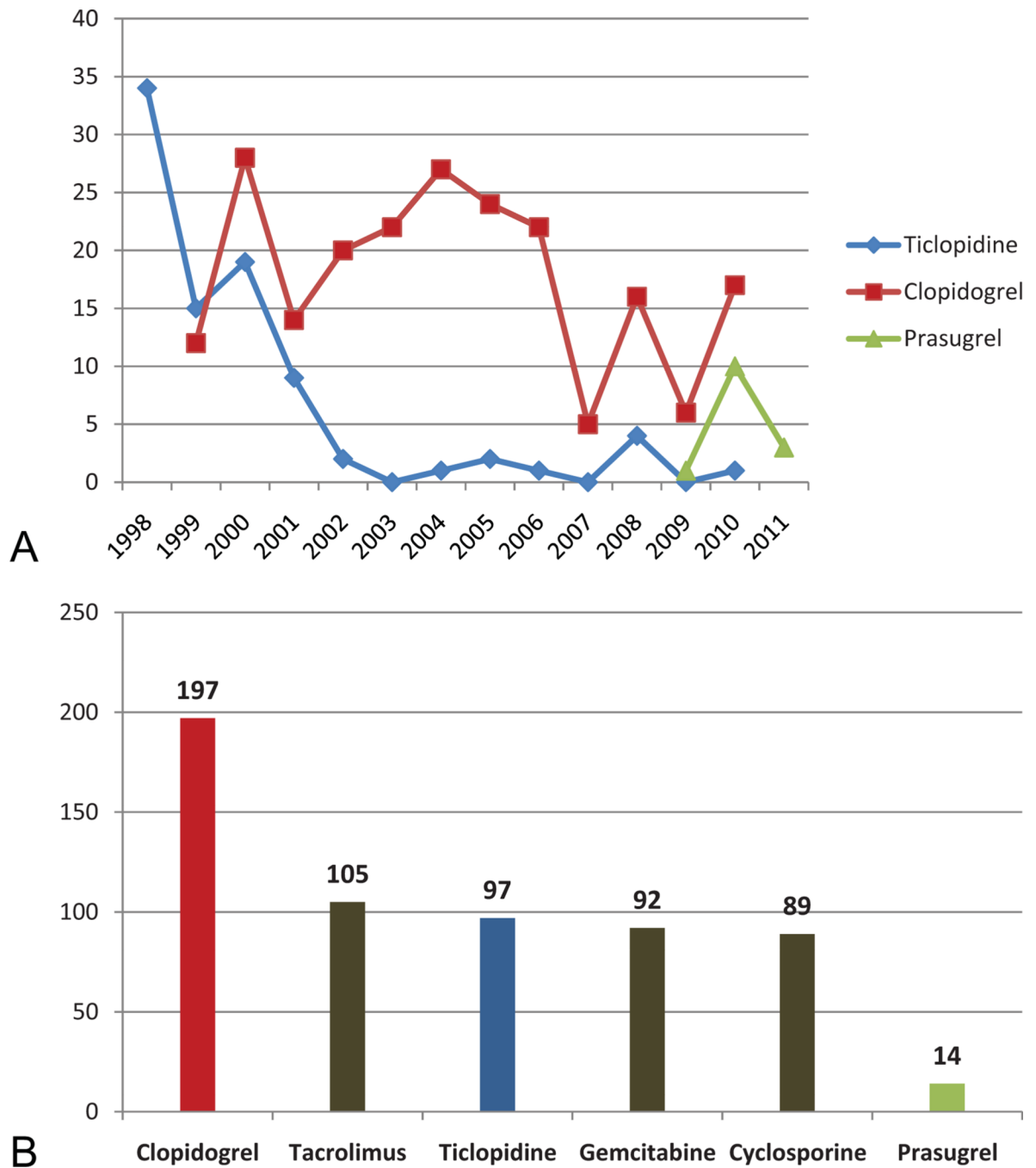
Fig. 2. A, Cases per year of thienopyridine-associated thrombotic thrombocytopenic purpura (TTP) reported to the U.S. Food and Drug Administration (FDA) (1998–2011). B, Drugs and number of cases reported to the FDA’s Adverse Event Reporting System in association with thrombotic thrombocytopenic purpura (1998–2011).
