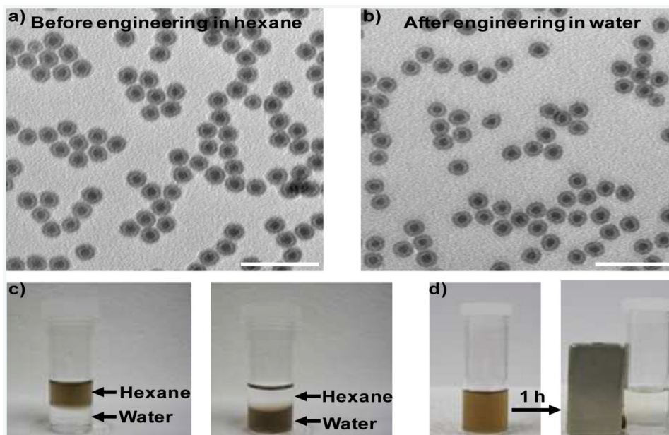
Figure 1. Characterization of chimeric DNA molecule-engineered Fe-Fe 3 O 4 CSNPs. TEM images of Fe-Fe 3 O 4 CSNPs a) before and b) after chimeric DNA molecule modification in hexane and water, respectively. c) Solvent dispersity of Fe-Fe 3 O 4 CSNPs before and after chimeric DNA molecule functionalization. The as prepared Fe-Fe 3 O 4 CSNPs are hydrophobic and disperse in hexane, while the functionalized Fe-Fe 3 O 4 CSNPs are hydrophilic and disperse in water. d) Magnetic separation of engineered Fe-Fe 3 O 4 CSNPs. Lipid-T20 was used as the chimeric DNA molecule here. Detailed sequence information for all the chimeric DNA molecules can be find in Table S1 (SI). Scale bars: 50 nm.
