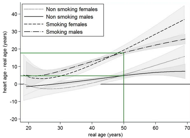
Figure 2 Heart age deviation in years (95% CI shown shaded in gray) for male and female smokers and non-smokers for real ages 20–70 years.
