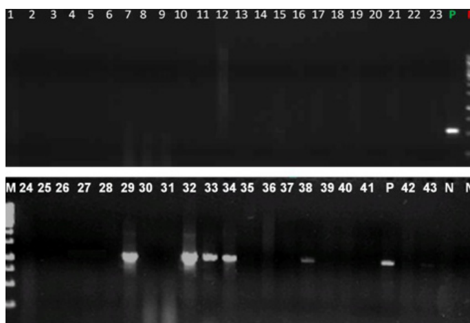
[Table/Fig-5]: PCR for bla TEM GENE
