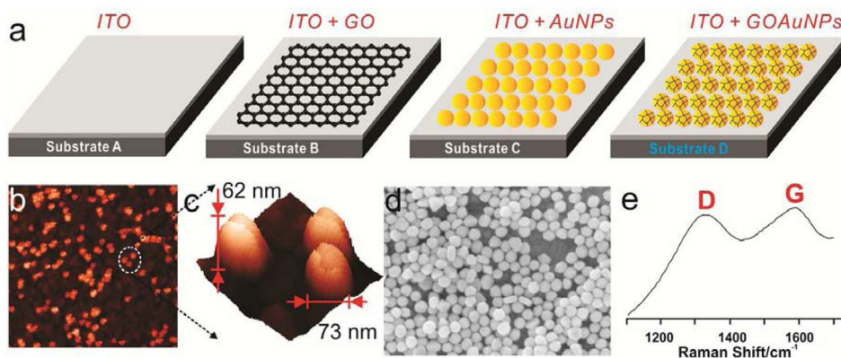
Figure 2. (a) Schematic diagram representing four different substrates modified with graphene (Substrate B), gold nanoparticles (Substrate C) and GO-encapsulated GNP (Substrate D). (b) AFM images of Substrate D and (c) high resolution AFM image of (b) for the confirmation of GO-encapsulated GNP nanoparticles. The X and Y axis were 3\mu\text{m} \times 3\mu\text{m} and 200\text{nm} \times 200\text{nm} for image (b) and (c), respectively, and the scan rate was 0.5Hz and 0.1Hz for image (b) and (c), respectively. (D) SEM image of Substrate D with a high concentrations of GO-encapsulated GNP. (e) Raman spectra of Substrate D to verify the encapsulation of GO on the surface of the GNPs.
