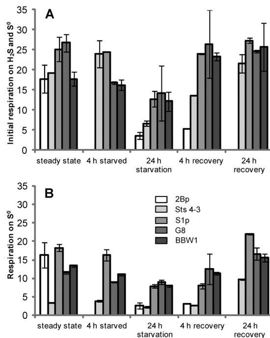
FIG 4 Effects of CS 2 starvation and recovery on respiration rates \pm the standard error of the mean ( n = 3 ) on internally produced H 2 S and S 0 (A) and on only S 0 (B) after a CS 2 pulse. The experiment was performed with five CS 2 -converting A. thiooxidans strains (2Bp, Sts 4-3, S1p, G8, and BBW1), all growing simultaneously in five identically run chemostats. Rates are given in nanomoles of O 2 per minute per milliliter of culture. Note that the respiration rates of strain 2Bp were monitored only at steady state, after 24 h of starvation, and after 4 h of recovery.
