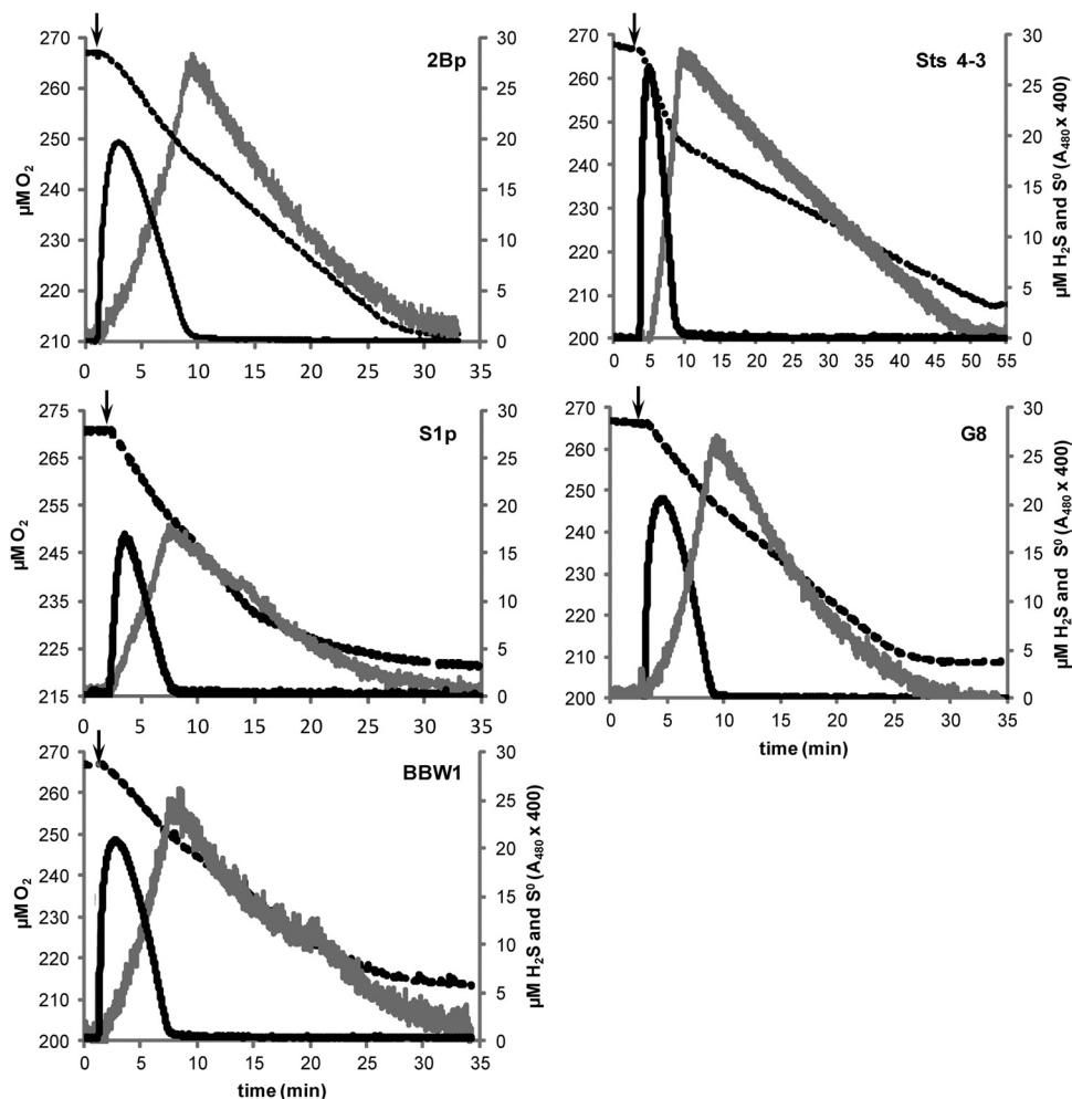
FIG 2 Conversion of \text{CS}_2 by five A. thiooxidans strains. The arrows indicate the times when 17 \mu\text{M} \text{CS}_2 was injected into a cuvette containing cells from a continuous culture growing at D = 0.02 , diluted 6\times in MM containing 1\% \text{H}_2\text{SO}_4 . Respiration ( \text{O}_2 consumption, black dashed line), \text{H}_2\text{S} production (black solid line), and \text{S}^0 production (gray line) were monitored. The production and consumption rates in these graphs were used to determine the percentages of \text{S}^0 accumulation in Table 2. Note the different scale on the x axis of the graph for strain Sts 4-3.
