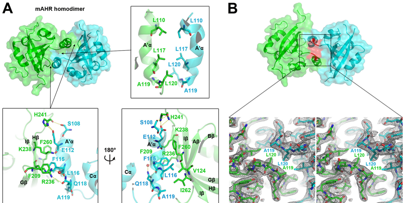
FIG 3 The details of the AHR PAS-A homodimer interface. (A) The interface is composed of two regions: between the two A'α-helices (top) and between one A'α-helix and the β-sheet (bottom). The interfacial residues are labeled and shown in sticks. Hydrogen bonds are indicated as yellow dashed lines, and water molecules are indicated as red dots. The secondary structure elements are labeled. (B) Ala119 and Leu120 locate at the central position of the AHR PAS-A dimer interface. The upper part is 180 degrees rotated from the AHR structure shown in panel A, with Ala119 and Leu120 colored in red. The lower one is a stereo image showing the detailed conformations of Ala119, Leu120, and residues around them in an electron density map (2Fo-Fc map contoured at 1.2 \sigma ).
