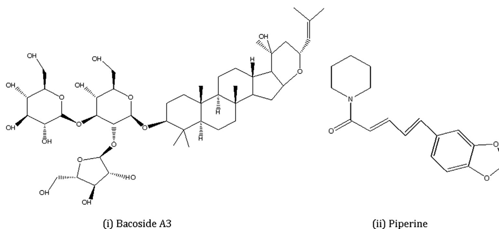
Fig. 1. Structure (i) Bacoside A 3 , (ii) Piperine.
