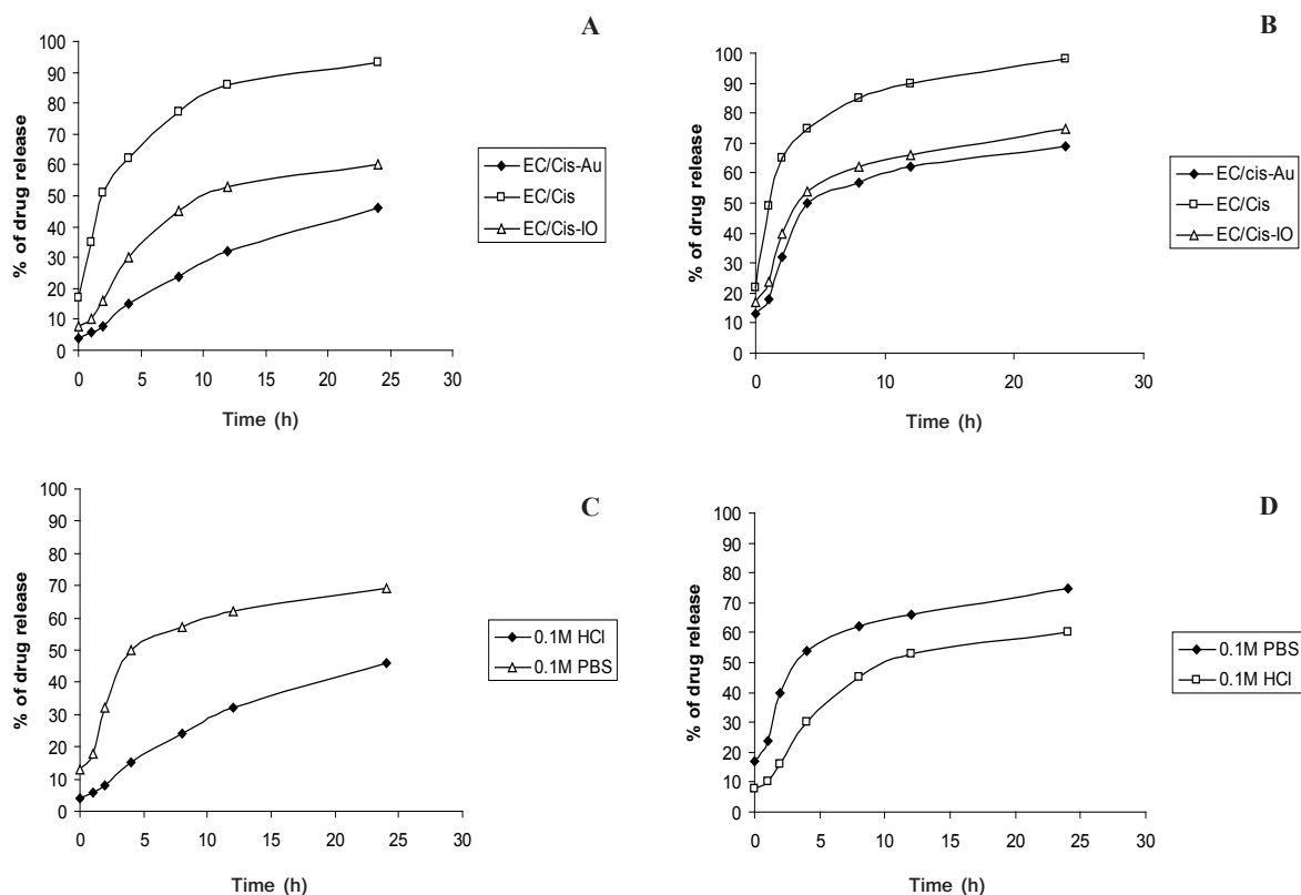
Figure 7. Drug release profiles of nanocapsules in (a) 0.1 M HCl (b) 0.1 M PBS. Drug release profiles using (c) gold nanoparticles (d) ironoxide nanoparticles.
