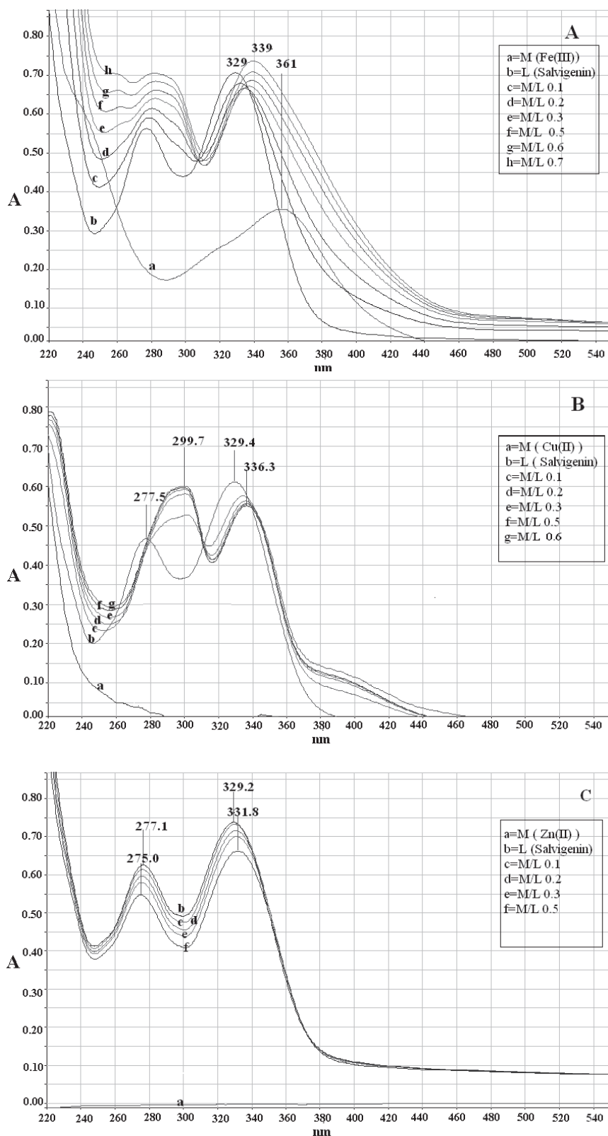
Figure 2. Electronic absorption spectra of (a) salviagenin ( 1.0 \times 10^{-4} M) in methanolic solution in absence and presence of Fe(III) without pH control, (b) salviagenin ( .0 \times 10^{-4} M) in methanolic solution in absence and presence of Cu(II) without pH control, (c) salviagenin ( .0 \times 10^{-4} M) in methanolic solution in absence and presence of Zn(II) without pH control.
