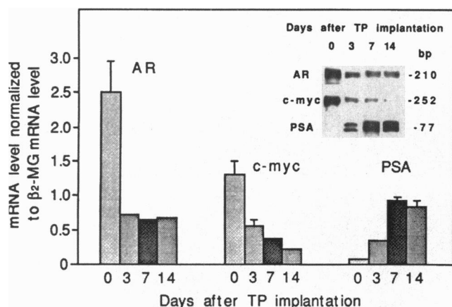
FIG. 7. The effect of TP on the expression of mRNAs for AR, c-myc , PSA, and \beta_2 microglobulin (MG) in LNCaP 104-R2 tumors. The autoradiogram from the RNase protection assay using ^{32} P-labeled antisense probes is shown in the Inset . The graphic represents quantitation of protected probes normalized to the amount of protected \beta_2 microglobulin probe. LNCaP 104-R2 cells were injected into castrated male nude mice, and 7 weeks after injection of cells, TP was implanted and tumors resected 0, 3, 7, and 14 days later for RNA extraction and RNase protection assay.
