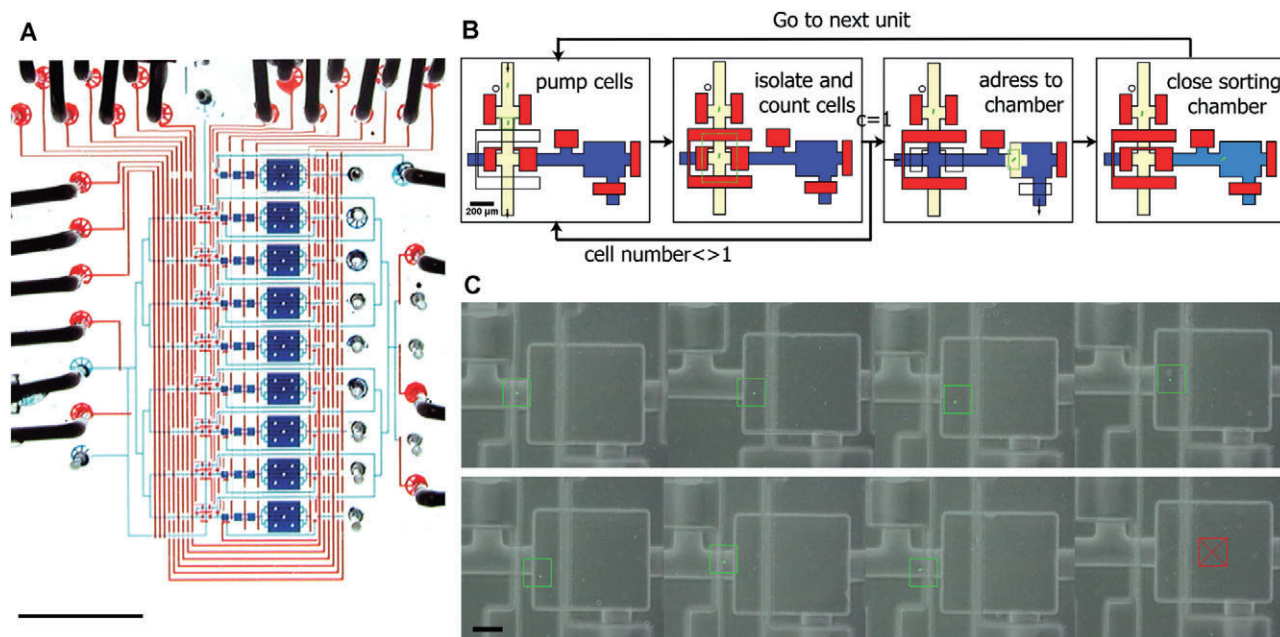
Fig. 1. Photograph of a single-cell isolation and genome amplification chip capable of processing nine samples in parallel (eight cells, one positive control). A. To visualize the architecture, the channels and chambers have been filled with blue food colouring and the control lines to actuate the valves have been filled with red food colouring (scale bar 5 mm). B. Schematic diagram of the automated sorting procedure. Closed valves are shown in red, open valves are transparent. Cells are drawn in green. C. Typical result of cell sorting showing for each unit (seven with a single cell and one negative control without a cell) a colour combination of a phase contrast image (gray) and a fluorescence image (green). A green overlaid square has been placed around the cell to ease visualization, whereas a red crossed square indicates the absence of cell. Scale bar is 100 \mu\text{m} . Reprinted from Marcy et al. (2007a).
