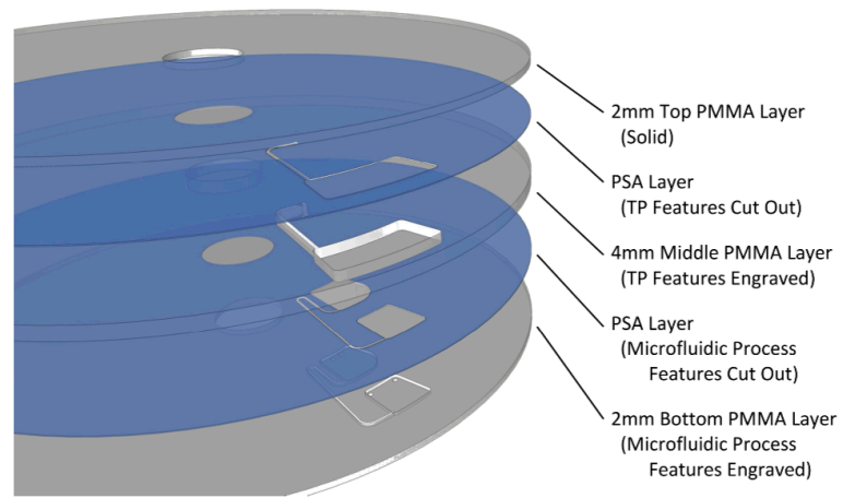
Fig. 2. Layered fabrication of the multi-level microfluidic CDs.
