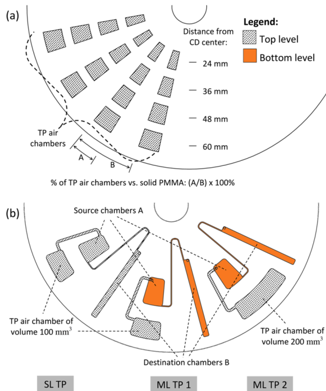
Fig. 4. (a) A design to evaluating CD surface heating. CD shown contains TP air chambers placed along various CD radii, and at 40% density (calculated by the percentage of area taken by TP air chambers on a radial path, denoted by (A/B) \times 100\% ). (b) CD designs to evaluated single-level TP pumping (SL TP), multi-level TP pumping (ML TP 1), and multi-level TP pumping with double volumed TP air chamber (ML TP 2).
