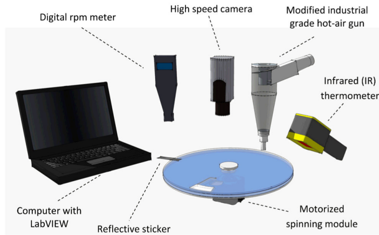
Fig. 3. Experimental setup: custom made CD spin test system consisting of a motorized spinning module, digital rpm meter, and high speed camera all controlled and monitored with a computer configured with LabVIEW. Forced convection heating and CD surface temperature measurement are performed using a modified industrial grade hot-air gun and infrared (IR) thermometer.
