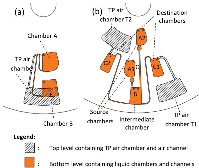
Fig. 5. (a) A design to demonstrate push-pull pumping. Liquid will be pushed from chamber A to B, and then pulled from chamber B to A (b) A design to demonstrate valve-less switch pumping. Liquid will burst from chamber A1 to B, then pulled into C1, followed by liquid bursting from chamber A2 to B, then pulled into C2.
