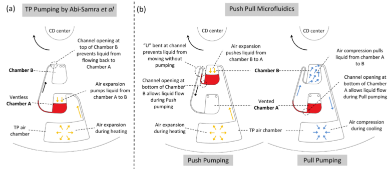
Fig. 1. (a) TP pumping by Abi-Samra et al. Ventless chamber A prevents incorporation of TP pumping in centrifugal driven microfluidic processes. (b) Push and Pull pumping principles. Design of "U" bent, location of channel opening at bottom of chambers, and vented chamber A allows incorporation of TP pumping as part of centrifugal driven microfluidic processes.
