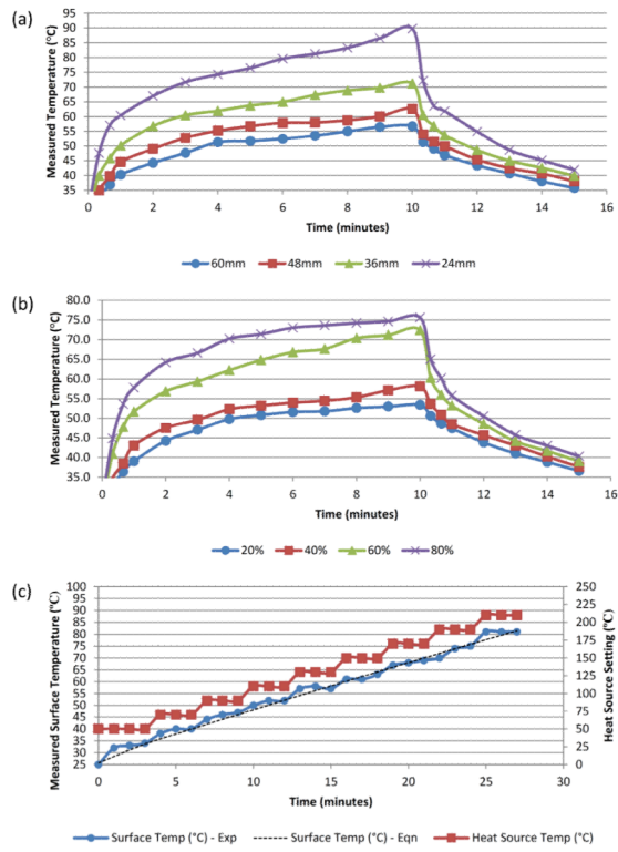
Fig. 6. (a) Heating pattern of CD surface with TP air chambers placed along various radii on the CD, at 40% density, 300rpm, and 190°C heating. (b) Heating pattern of CD surface with TP air chambers of various density, placed along 60mm radius, at 300rpm, and 190°C heating. (c) Achievable CD surface temperature with stepped increments of heat source setting.
