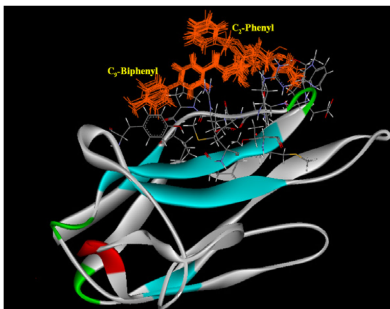
Figure 2. View of the simulated representative structure of compound 5 bound to the mCD22. Structures colored in grey are protein residues.
