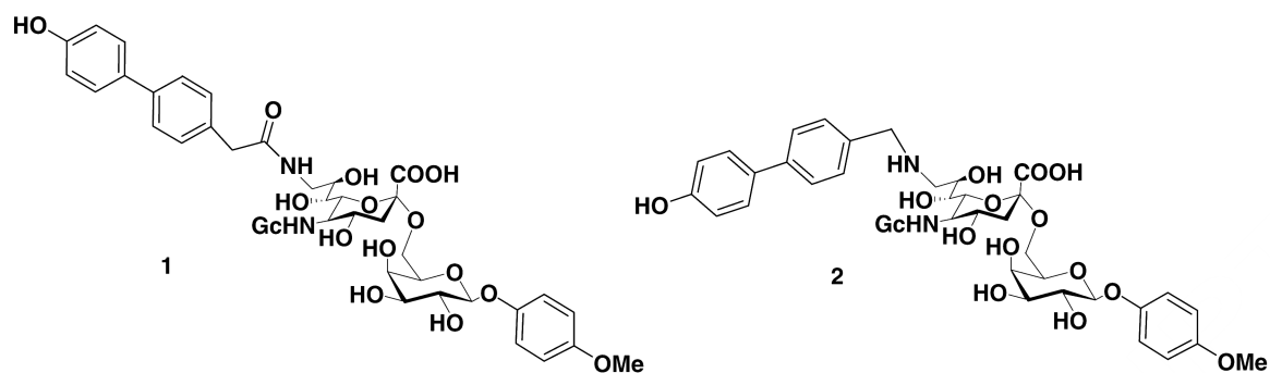
Figure 1. Structures of the 9-amido ( 1 ) and 9-amino ( 2 ) sialosides. 6
