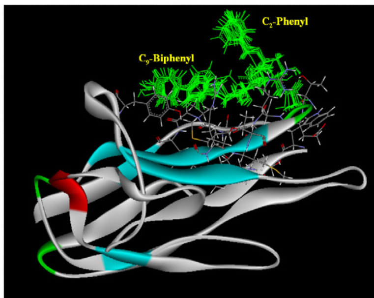
Figure 3. View of the simulated representative structure of compound 8 bound to the mCD22. Structures colored in grey are protein residues.
