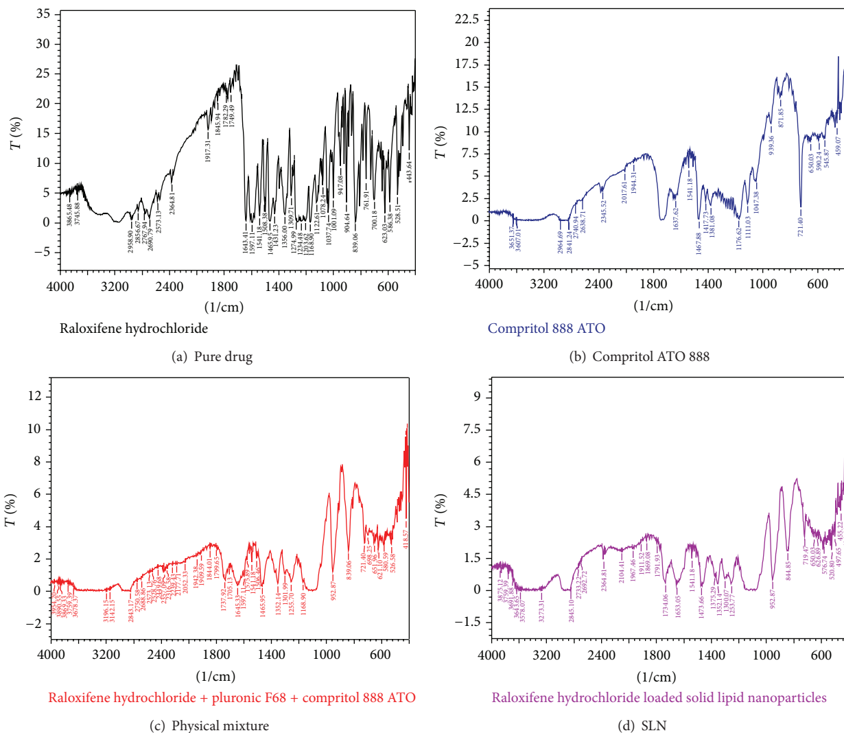
FIGURE 5: FTIR spectra.
