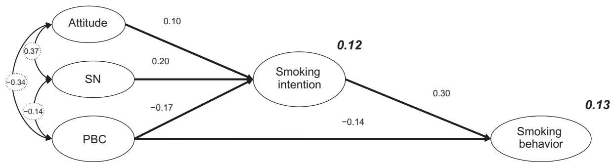
Figure 2 MASEM analysis.
