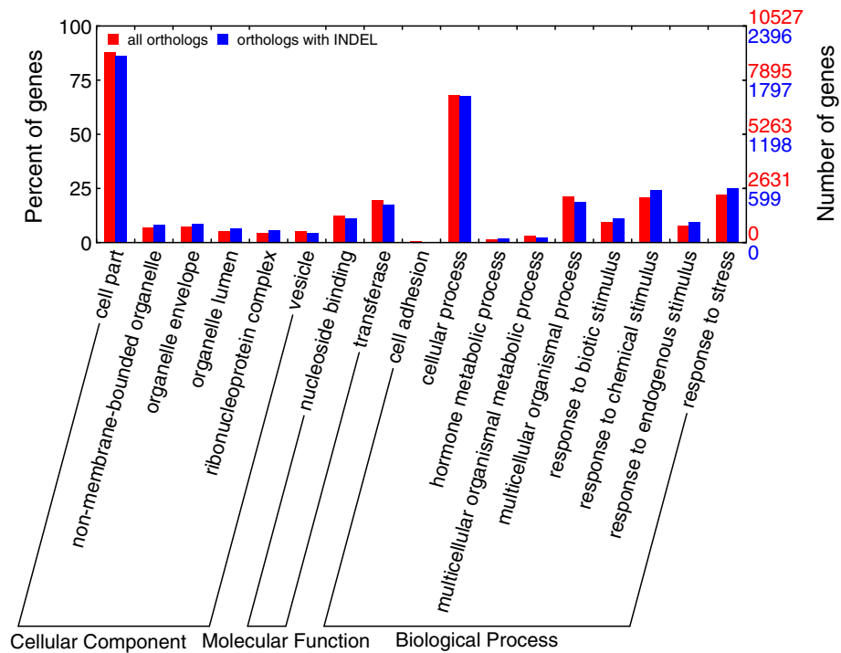
Figure 6 GO enrichment on orthologs with INDEL. Direct parent GO terms in biological process domain are displayed for simplicity. The GO terms in the biological process domain that show increase in ESTs with INDEL are related to hormone metabolic process and response to various stimuli (including response to stress).
