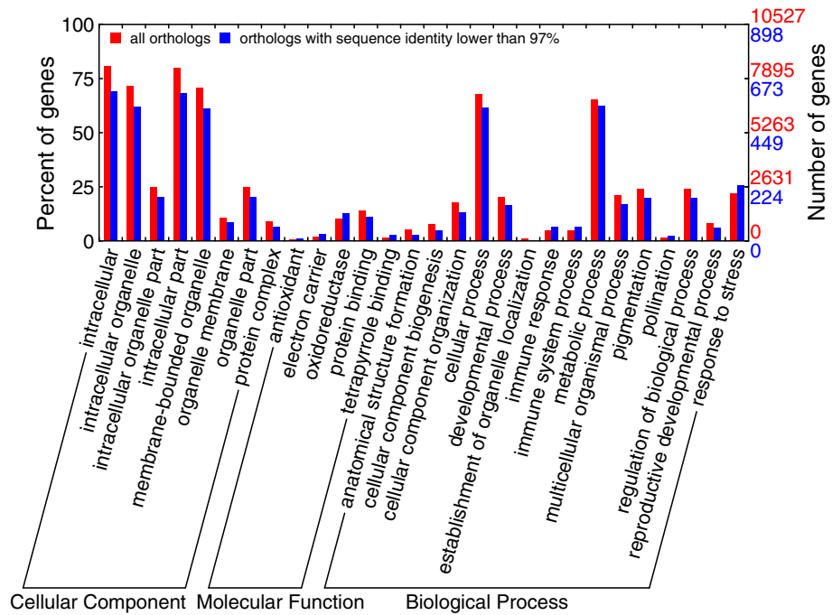
Figure 5 GO enrichment on orthologs with sequence identity lower than 97%. Direct parent GO terms in biological process domain are displayed for simplicity. The GO terms in the biological process domain that show increase in ESTs with lower sequence identity are related to immune response and response to stress.
