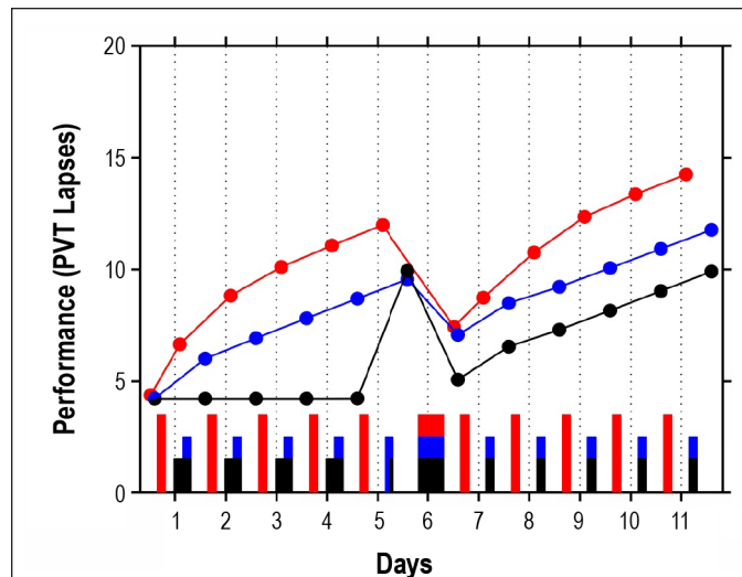
Figure 7 —Model predictions for the effects of sustained sleep restriction comparing hypothetical schedules with nighttime versus daytime sleep and different sleep histories. The blue trajectory displays predicted performance (PVT lapses) for a scenario beginning with 5 days with 4 h nocturnal sleep (TIB: 03:30-07:30) and ending with a recovery day with 12 h nocturnal sleep (TIB: 19:30-07:30) followed by 5 days with 4 h nocturnal sleep (TIB: 03:30-07:30). The black trajectory displays predicted performance for a scenario also ending with a recovery day with 12 h nocturnal sleep and 5 days with 4 h nocturnal sleep, but beginning with 4 days with 8 h nocturnal sleep (TIB: 23:30-07:30) followed by a day with only a 1.5 h nap (TIB: 06:00-7:30). The red trajectory shows predicted performance for a scenario beginning with 5 days with 4 h diurnal sleep (TIB: 15:30-19:30) and ending with a recovery day with 12 h nocturnal sleep (TIB: 19:30-07:30) followed by 5 days with 4 h diurnal sleep (TIB: 15:30-19:30), where circadian phase adjustment is assumed to be negligible. In all three scenarios, baseline sleep is assumed to involve 8 h TIB at night (23:30-07:30) for several days prior. Dots represent averages across the interval from 2 h to (up to) 12 h after scheduled awakening for each period of wakefulness. Bars indicate sleep periods.
