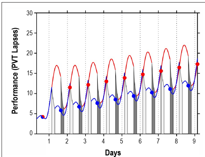
Figure 6 —Model predictions for the effects of sustained sleep restriction on neurobehavioral performance when wakefulness is placed during the night as compared to during the day. The blue trajectory displays predicted performance (PVT lapses) across days with 20 h diurnal wakefulness and 4 h nocturnal sleep (dark gray bars; TIB: 03:30-07:30). The red trajectory displays predicted performance across days with the restricted sleep periods shifted 12 h later, i.e., with 20 h nocturnal wakefulness and 4 h diurnal sleep (light gray bars; TIB: 15:30-19:30). In both scenarios, baseline sleep is assumed to involve 8 h TIB at night (23:30-07:30) for several days prior. In agreement with preliminary laboratory findings, 66 circadian phase adjustment in the shifted scenario is assumed to be negligible. Circadian effects on sleep efficiency are accounted for in the model dynamics. Dots represent averages across the interval from 2 h to 14 h after scheduled awakening for each period of wakefulness.
