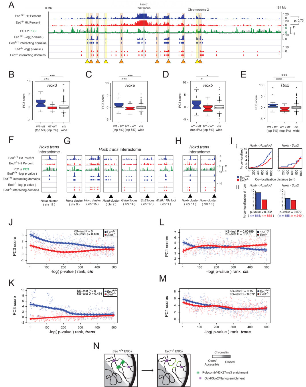
Figure 7. Eed is required for the co-localization of Polycomb-occupied genomic regions
