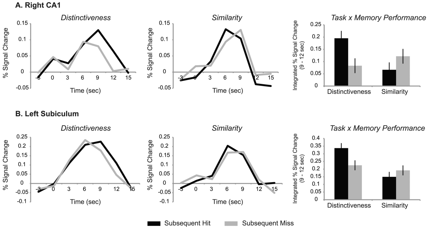
Figure 6. Encoding task by subsequent memory interaction. Timecourses represent encoding activity associated with subsequent hits and misses for the Distinctiveness and Similarity tasks. Bar graphs represent integrated percent signal change from 9–12 sec. Encoding activity in right CA1 (A) and left subiculum (B) revealed a significant interaction between encoding task and subsequent memory late in the timecourse, such that greater subsequent memory effects were observed for the Distinctiveness than the Similarity task (right CA1, p = .016 ; left subiculum, p = .047 ).
