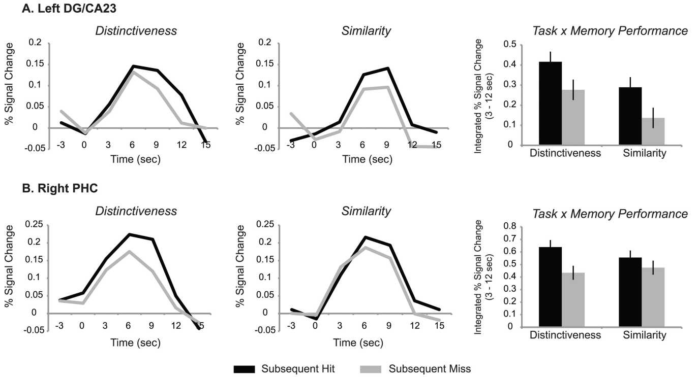
Figure 5. Main effect of subsequent memory. Timecourses represent encoding activity associated with subsequent hits and misses for the Distinctiveness and Similarity tasks. Bar graphs represent integrated percent signal change from 3–12 sec. Encoding activity in left DG/CA 2/3 (A) and right parahippocampal cortex (B) revealed a main effect of subsequent memory such that collapsed across task, activity associated with subsequent hits was greater than that for misses (left DG/CA 2/3 , p = .004 ; right parahippocampal cortex, p = .002 ). DG: dentate gyrus. PHC: parahippocampal cortex.
