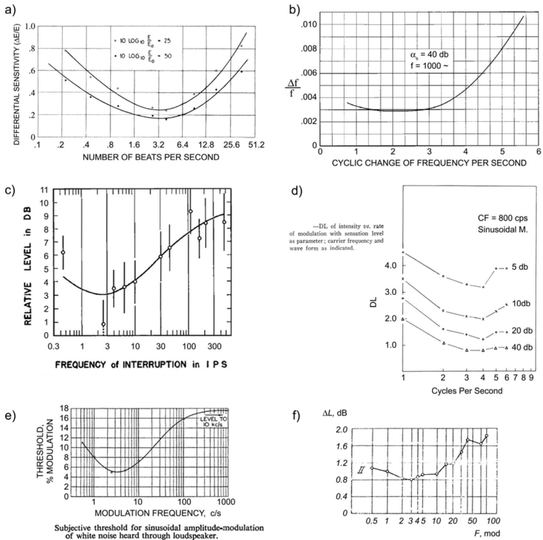
Figure 4. Historical demonstrations of maximum sensitivity to modulations in the range ~2-5 Hz. See text for info. a) Riesz (1928), beats (SAM tones). b) Shower and Biddulph (1931), FM tones. c) Pollack (1951), interrupted white noise. d) Tonndorf et al. (1955), SAM tones. e) Stott and Axon (1955), SAM white noise. f) Dubrovskii and Tumarkina (1967), SAM white noise.
