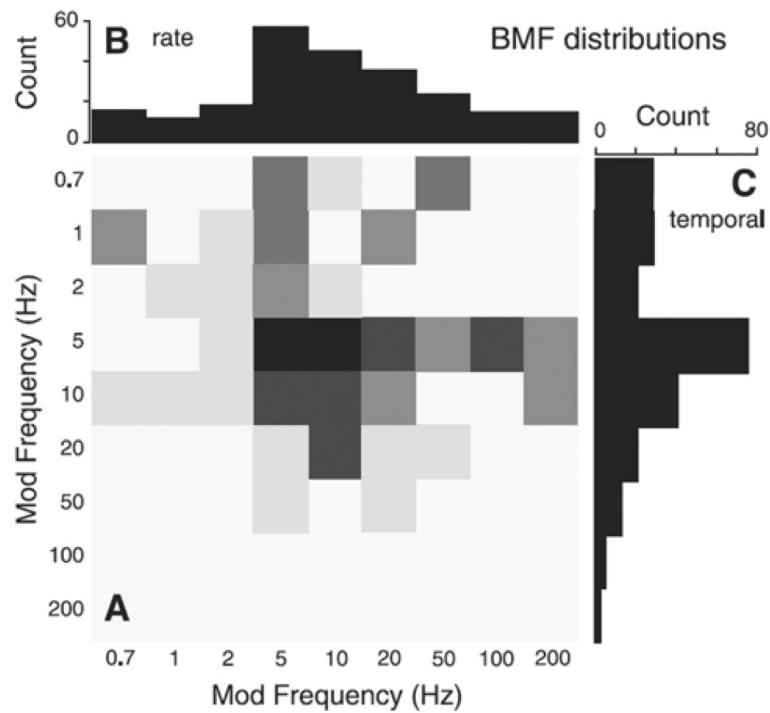
Figure 13. Single-unit responses to SAM tones in AI of unanesthetized monkey (Malone et al. 2007). For each single-unit, a best modulation frequency (BMF) was calculated either based on overall firing rate increase (B) or on a temporal measure (C). Both measures indicate a peak at ~5-10 Hz, with the majority of BMFs found in the range ~4-32 Hz. The joint distribution (A, 361 AI neurons total) shows that the two measures are roughly, but not perfectly, correlated.
