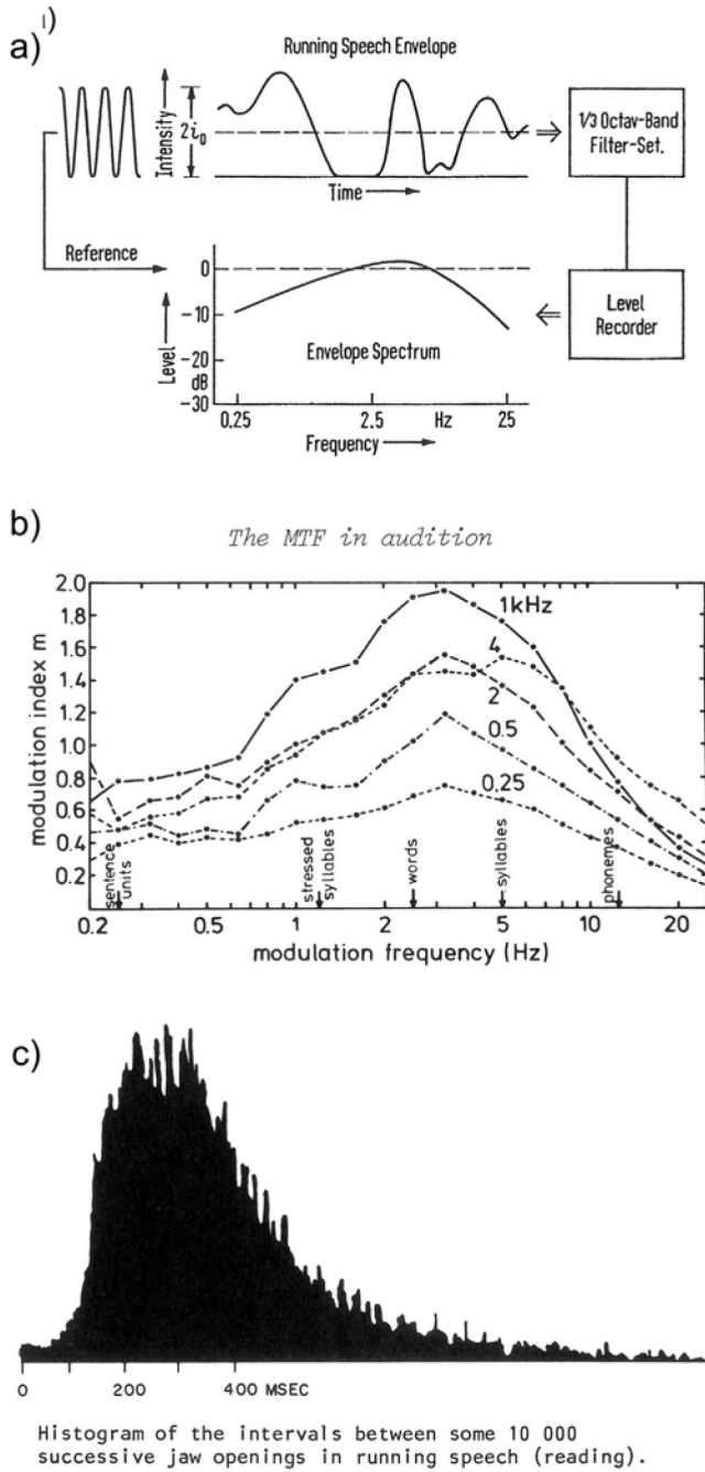
Figure 5. The envelope spectrum of natural speech production. a) Houtgast and Steeneken (1973): “The fluctuations of running speech as represented by the envelope spectrum.” b) Plomp et al. (1984): Average envelope spectrum for 1-min discourses from 10 male speakers. c) Ohala (1975): Jaw opening intervals during continuous speech. The majority of intervals occur in the range ~200-500 ms (i.e., ~2-5 Hz) and almost all intervals (other than small motion noise discussed by the author) occur in the range ~100-1000 ms (~1-10 Hz).
