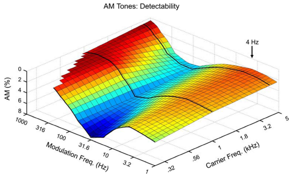
Figure 3. Detectability of AM tones as a function of f_c and f_m according to data of Zwicker (1952), which is the most complete to date. Three f_c s were tested (0.25, 1 and 4 kHz), as indicated by the black curves, over a wide range of f_m s. Further details are given in the text. The major result for present purposes is the peak in sensitivity centered at f_m = 4 Hz. Note also the overall increase in sensitivity in going to toward the basal region of the cochlea (higher f_c s), which play an overall stronger role in temporal envelope processing.
