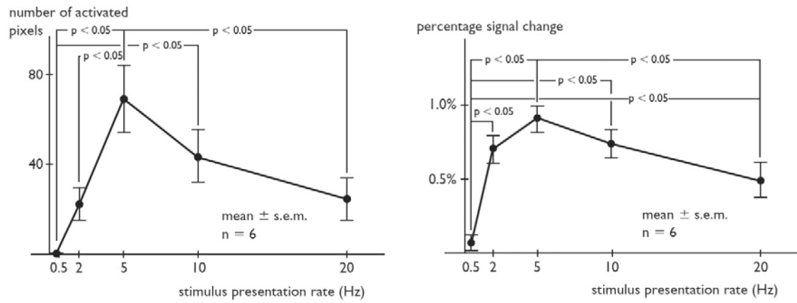
Figure 8. fMRI results of Tanaka et al. (2000), using a sinusoidally-AM tone. Note that both the activation extent (left) and strength (right) increase near ~5 Hz. This figure concerns primarily HG, and can be compared favorably with monkey single-unit results below (Malone et al., 2007) (Section 5).
