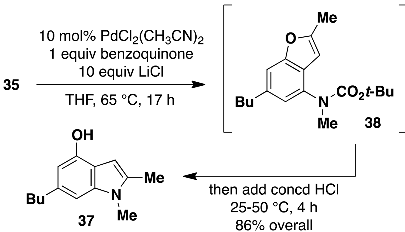
Scheme 5. Indole Synthesis via Hegedus Cyclization: An Alternative Route
