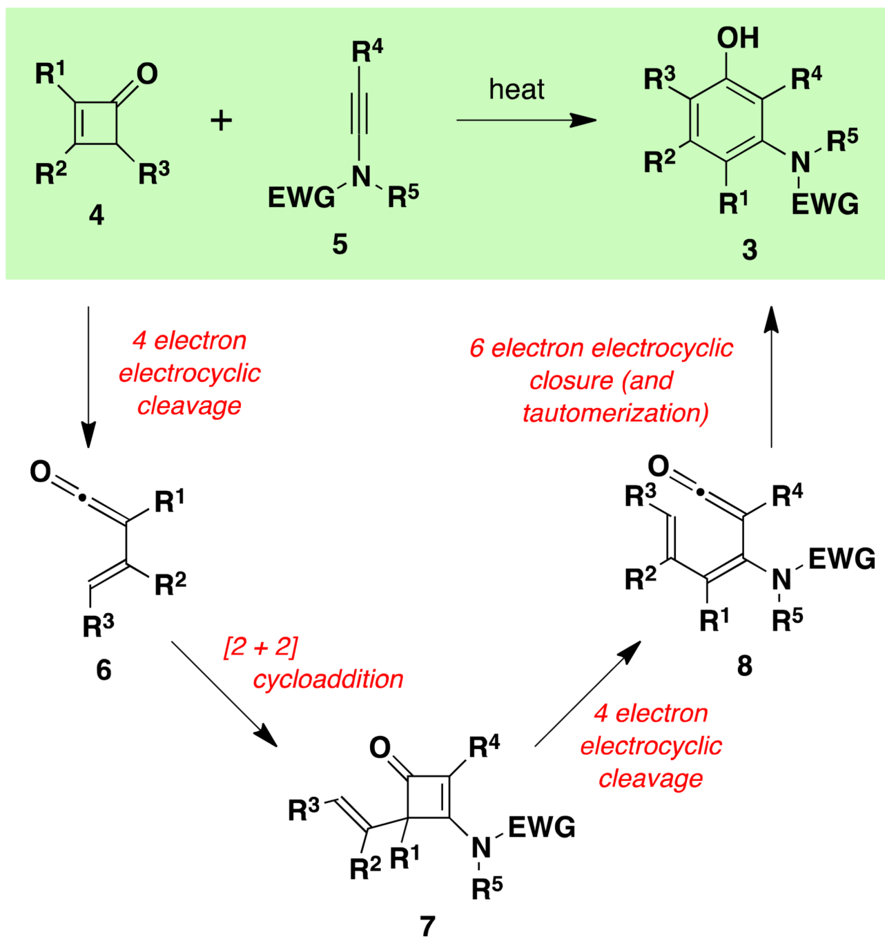
Scheme 2. Pericyclic Cascade Mechanism of the Vinylketene-Based Benzannulation
