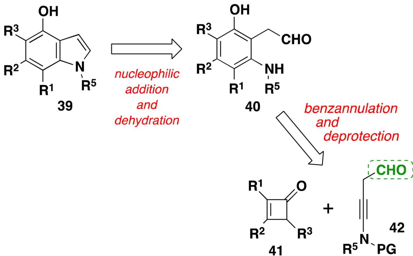
Scheme 6. Strategy for the Synthesis of Indoles via Aminobutynal Derivatives
