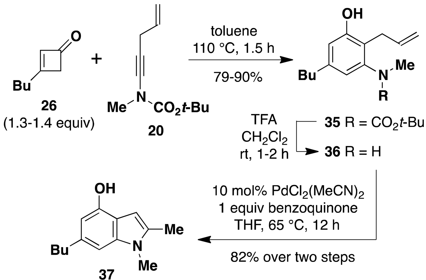
Scheme 4. Synthesis of Indole 37 via Benzannulation and Hegedus Cyclization
