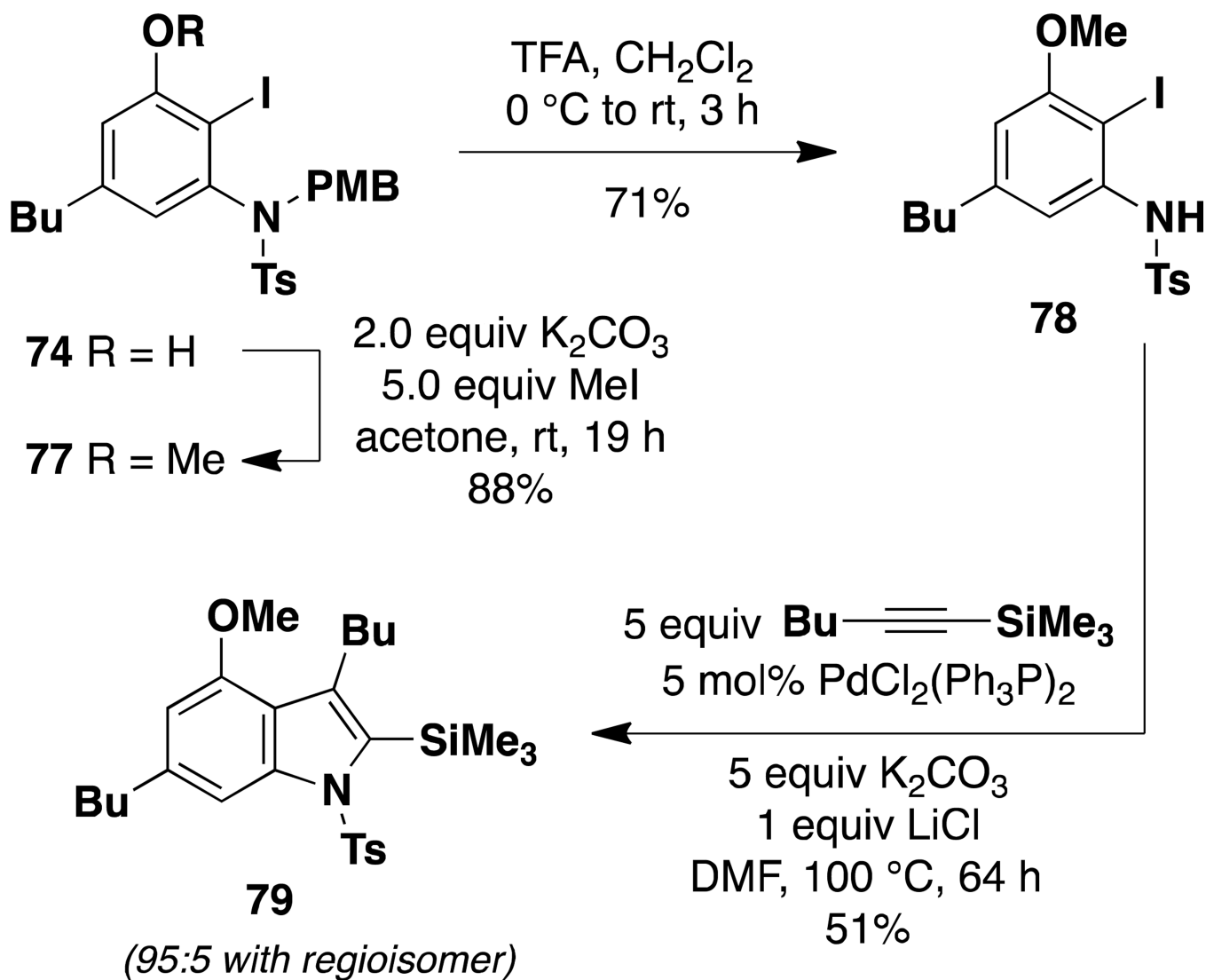
Scheme 11. Synthesis of Indole 79 via Larock Heteroannulation
