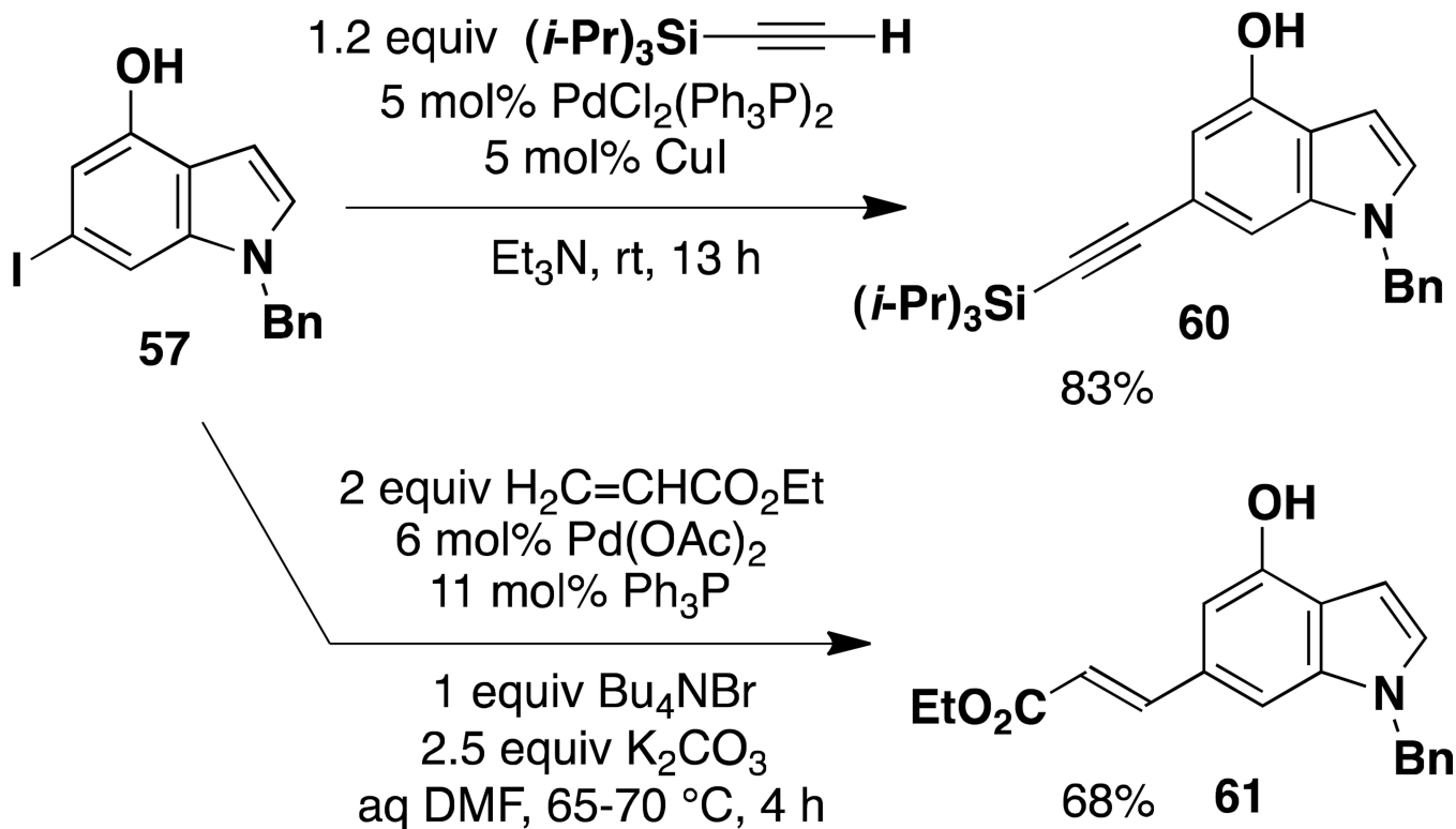
Scheme 8. Cross-coupling Reactions of 6-Iodoindole 57
