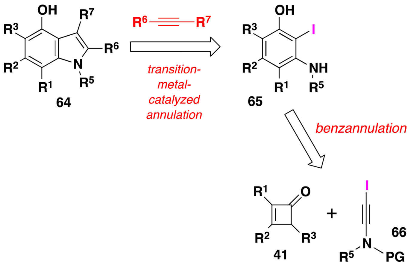
Scheme 10. Strategy for the Synthesis of Indoles via Iodoamides
