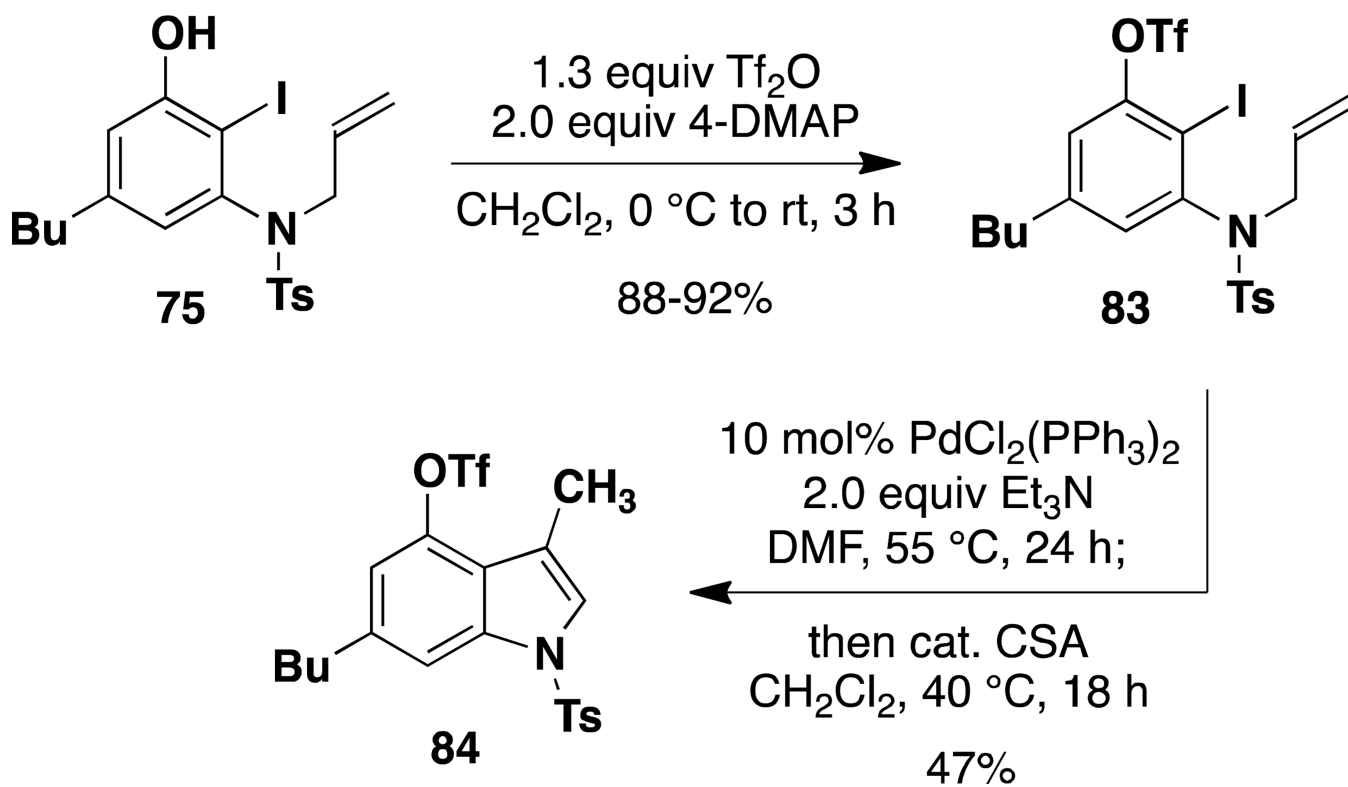
Scheme 13. Synthesis of Indole 84 via Mori-Ban Cyclization
