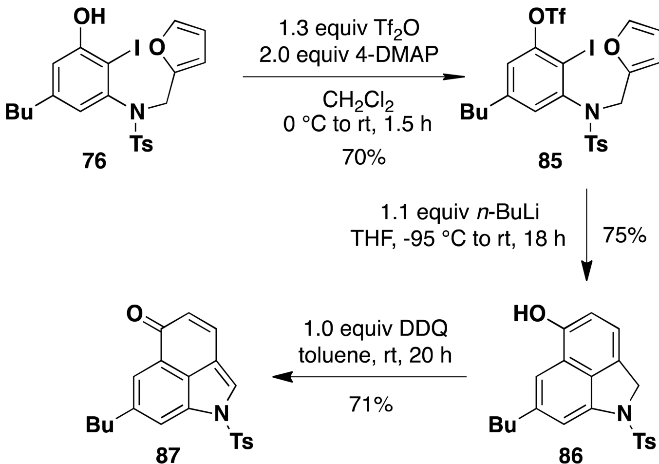
Scheme 14. Intramolecular Aryne Cyclization and Oxidation from Aniline 76
