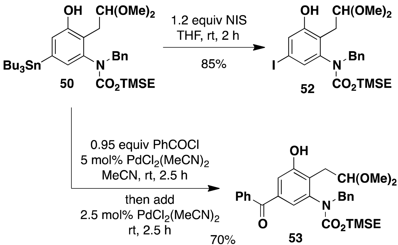
Scheme 7. Elaboration of Arylstannane 50
