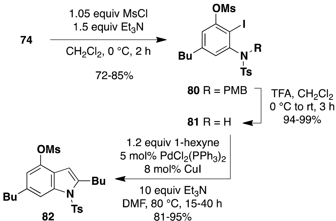
Scheme 12. Synthesis of Indole 82
