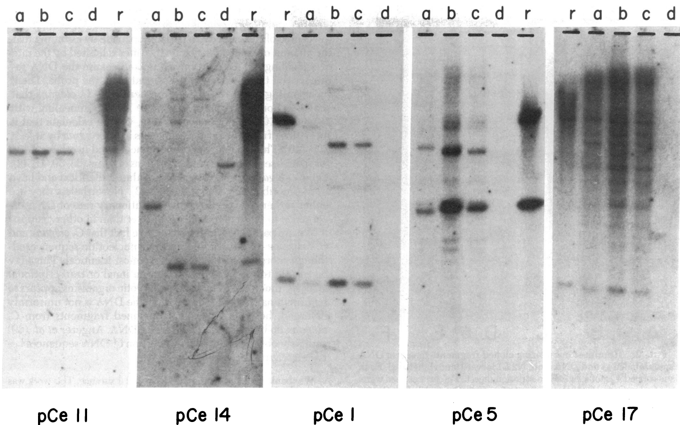
FIG. 1. Results of hybridizing five recombinant plasmids to DNA from L1 larvae of C. elegans var. Bergerac (a), DNA from L1 larvae of C. elegans var. Bristol (N2) (b), DNA from young adult hermaphrodites of C. elegans var. Bristol (N2) (c), mixed worms of C. briggsae (d), and a reconstruction to show the size of the fragment used as probe (r). Lanes a–d have approximately 2 \mu g of DNA from a Bam HI restriction digest. In each case the reconstruction consisted of 5 \mu g of sheared E. coli DNA plus 0.1 ng of plasmid to be used as probe, cleaved with Bam HI. Because the C. elegans genome consists of 8 \times 10^7 base pairs (12), 2 \mu g of worm DNA will contain 0.1 ng of a restriction fragment 4000 base pairs long. Hybridization in the reconstruction lane is to the cloned nematode fragment, to the pBR313 vector plasmid, and to the E. coli DNA (the last resulting from contamination of the radioactive probe with E. coli sequences). The sizes of the cloned fragments are as follows: pCe11, 5300 base pairs; pCe14, 2400 and 450 base pairs (two inserts); pCe1, 1800 base pairs; pCe5, 3750 base pairs; pCe17, 1650 base pairs.
