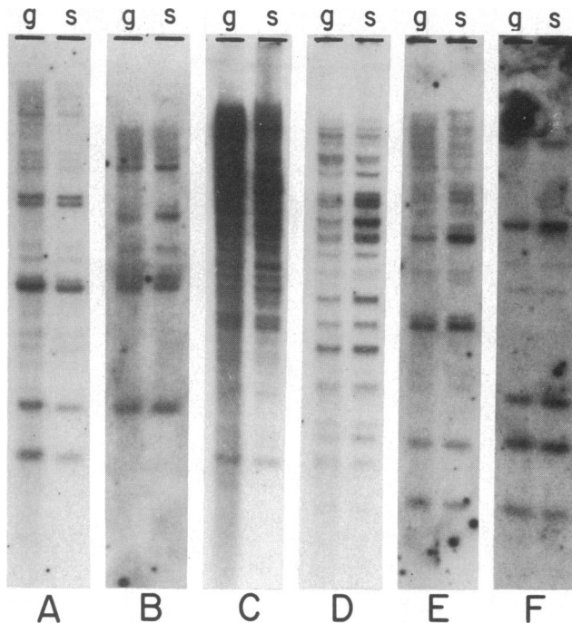
FIG. 2. Results of hybridizing cloned fragments to sperm DNA (lanes labeled g) and DNA from N2 L1 larvae (lanes labeled s). Each lane carried 4 \mu g of a Bam HI restriction digest. The probes used were: A, pCe1, pCe4, pCe5; B, pCe2, pCe3, pCe5; C, pCe17; D, pCe18a, pCe18b; E, pCe1, pCe10, pCe14; and F, pCe5, pCe13, pCe19.
