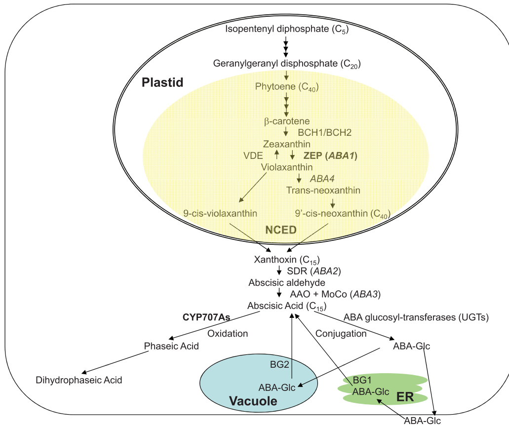
Figure 3. ABA metabolic pathways.
