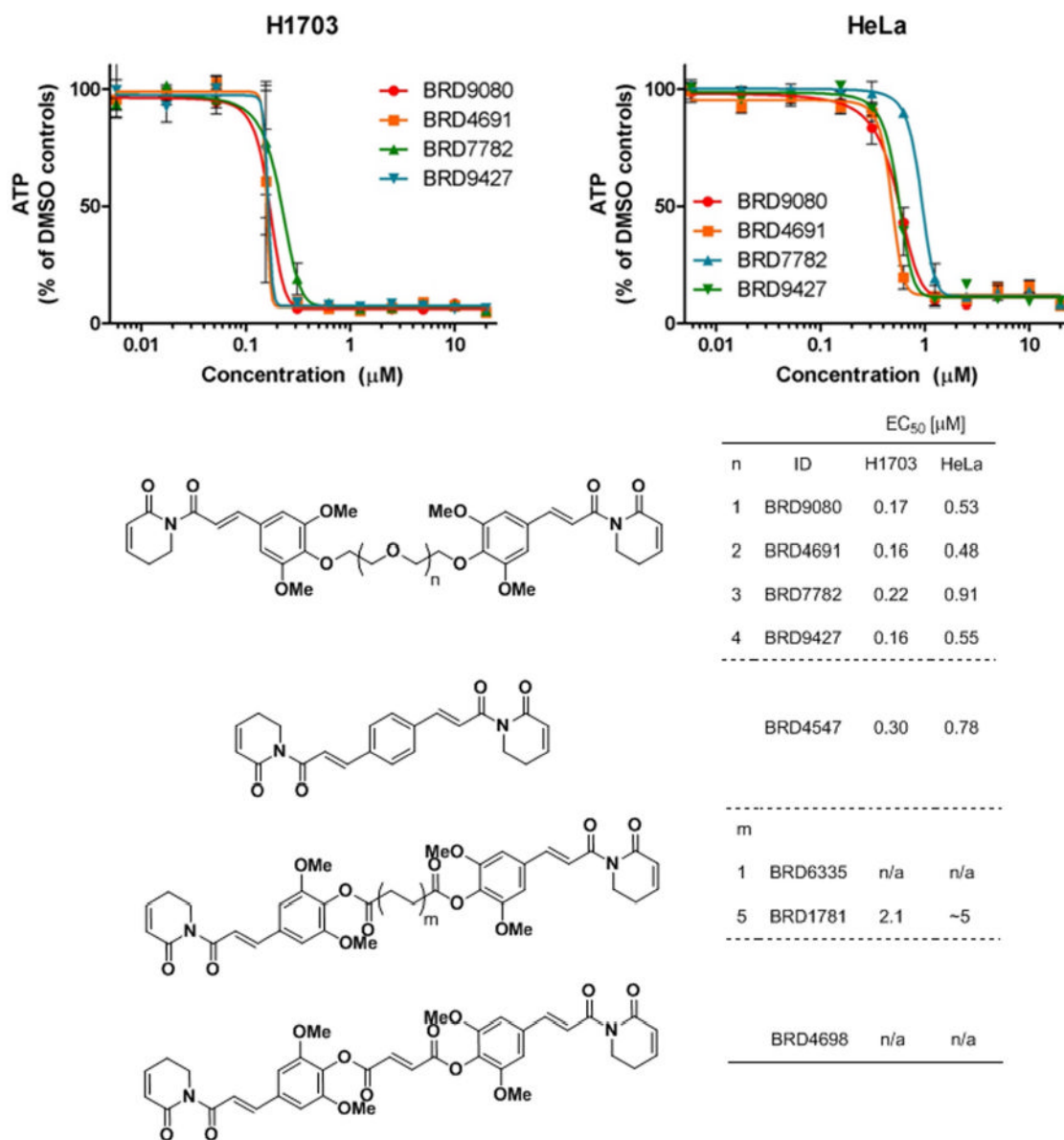
Figure 2. EC 50 values of tethered 'dimeric' imide-containing piperlogs in H1703 and HeLa cell lines. All data are expressed as mean \pm standard deviation for three independent experiments.
