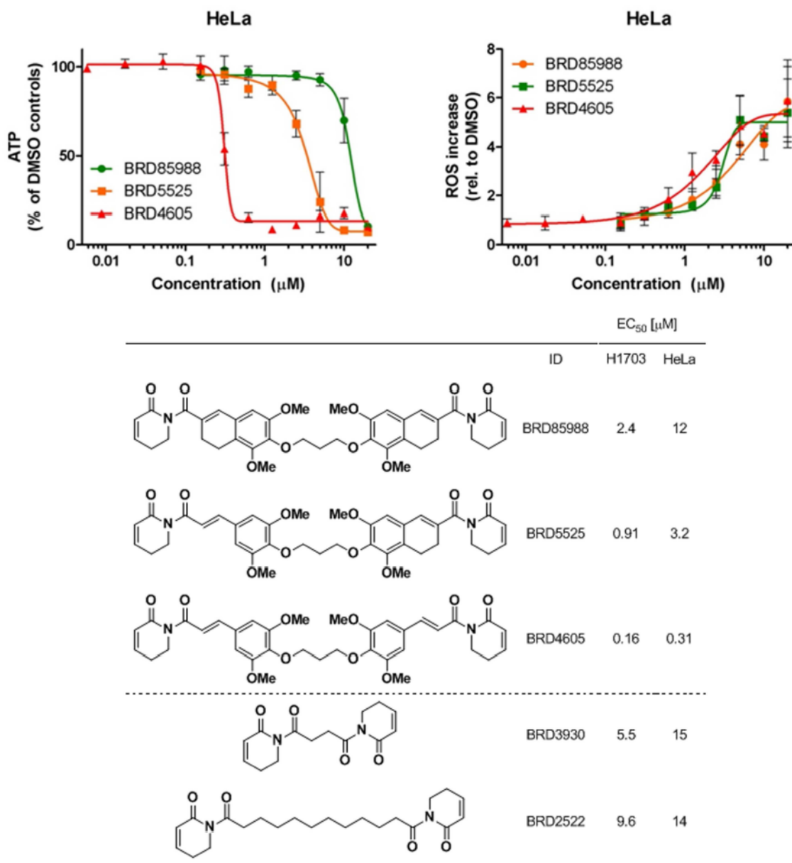
Figure 3. Viability (top left) and ROS increase (top right) of 'dimeric' piperlogs with C7-C8 olefin modifications determined from three independent experiments. All data are expressed as mean \pm standard deviation for three independent experiments.
