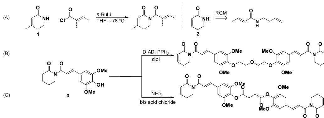
Scheme 1. Synthetic procedures for the preparation of piperlogs.
