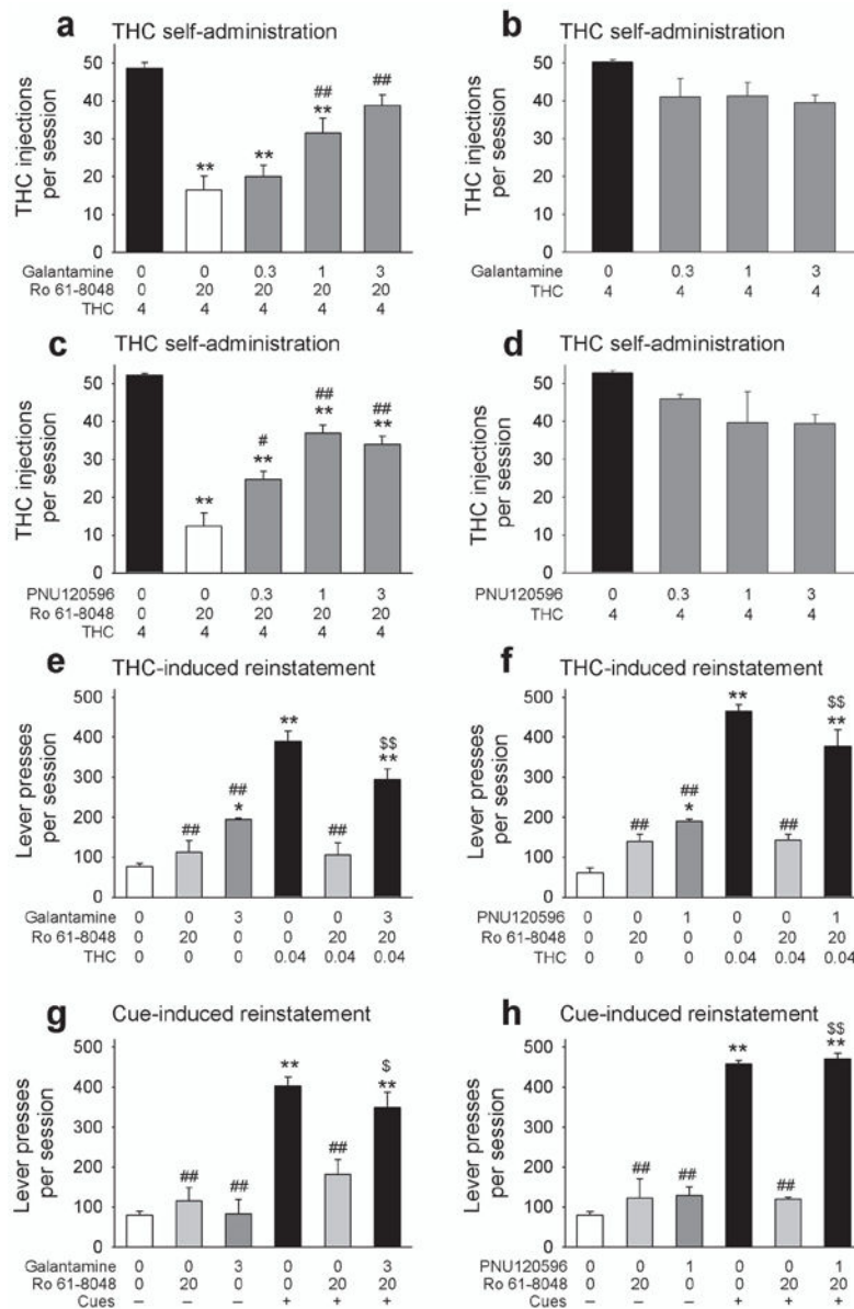
Figure 6. Reversal of behavioral effects of Ro 61-8048 by positive allosteric modulators of \alpha 7 nAChRs. Galantamine (a) or PNU120596 (c) dose-dependently reversed the blockade of THC (4 \mu g per kg per injection) self-administration caused by pretreatment with Ro 61-8048 (20 mg per kg). Galantamine (b) and PNU120596 (d) alone had no significant effect. **P < 0.01 , post-hoc vs. vehicles + THC 4; ##P < 0.01 , post-hoc vs. vehicle + Ro 20 + THC 4, Tukey test. (e,f) Treatment with Ro 61-8048 blocked the reinstatement of extinguished THC-seeking responses produced by a priming injection of THC (0.04 mg per kg i.v.), and this effect was prevented by pretreatment with galantamine (e) or PNU120596 (f). **P < 0.01 , post-hoc vs. vehicles; ##P < 0.01 , post-hoc vs. vehicles + THC 0.04, $$P < 0.01 , post-hoc vs. vehicle + Ro 20 + THC 0.04, Tukey test. (g,h) Treatment with Ro 61-8048 also blocked the reinstatement of extinguished THC-seeking responses induced by reintroduction
