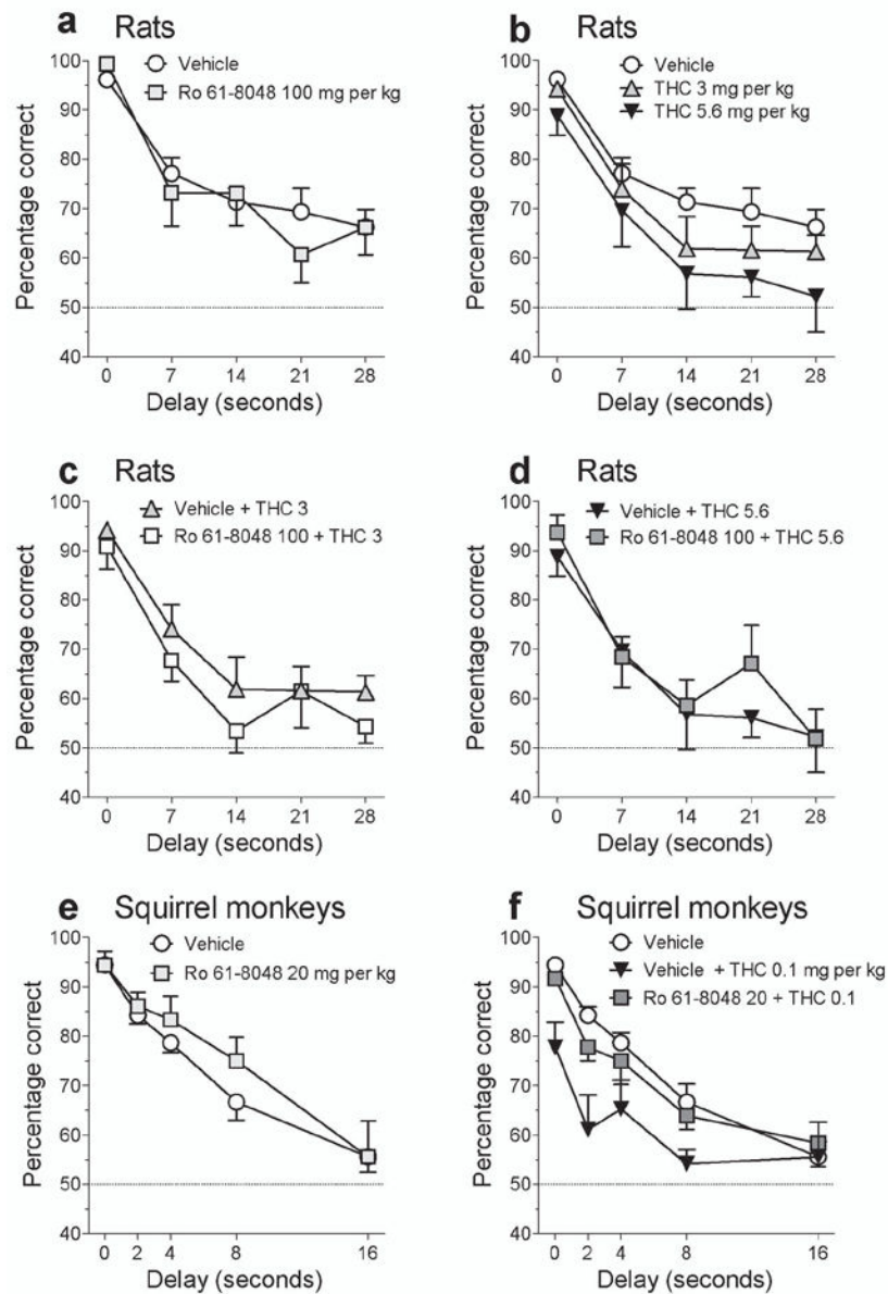
Figure 7. Effects of Ro 61-8048 and THC on working memory in rats and squirrel monkeys. (a-d) The 100 mg per kg dose of Ro 61-8048, which was effective in blocking the effects of THC in reward-related brain areas in rats, did not have deleterious effects on short-term memory in rats when given alone (a) or in combination with THC (3 or 5.6 mg per kg i.p.) (c,d) in a delayed nonmatching-to-position model of working memory. Both doses of THC significantly decreased accuracy (b) ; P 's < 0.007, but this was not exacerbated by Ro 61-8048 (c,d) . (e,f) The 20 mg per kg dose of Ro 61-8048, which was effective in blocking the effects of THC in reward-related brain areas in monkeys, did not have deleterious effects on short-term memory in monkeys when given alone (e) or in combination with THC (f) in a delayed matching-to-sample model of working memory. THC (0.1 mg per kg i.m.) significantly decreased accuracy (f) , and this was reversed by Ro 61-8048 (f) . Accuracy
