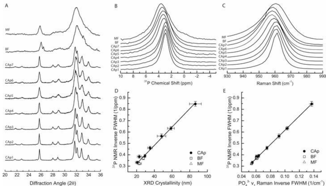
Figure 1. X-ray diffraction, ^{31}\text{P} NMR, and Raman spectral analysis of synthetic carbonated apatites in the 0.3–10.3 wt% range (CAp1–CAp7, ordered from low to high \text{CO}_3^{2-} content), bovine femur (BF), and mouse femur (MF) powdered bone samples. A) XRD patterns normalized to c-axis reflection (002). B) Normalized ^{31}\text{P} NMR spectra and C) normalized Raman spectra of \text{PO}_4^{3-} . D) X-Y plot of ^{31}\text{P} NMR inverse FWHM versus XRD crystallinity with x and y error bars representing standard deviation. E) X-Y plot of ^{31}\text{P} NMR inverse FWHM versus Raman \text{PO}_4^{3-} inverse FWHM. X and y error bars represent standard deviations.
