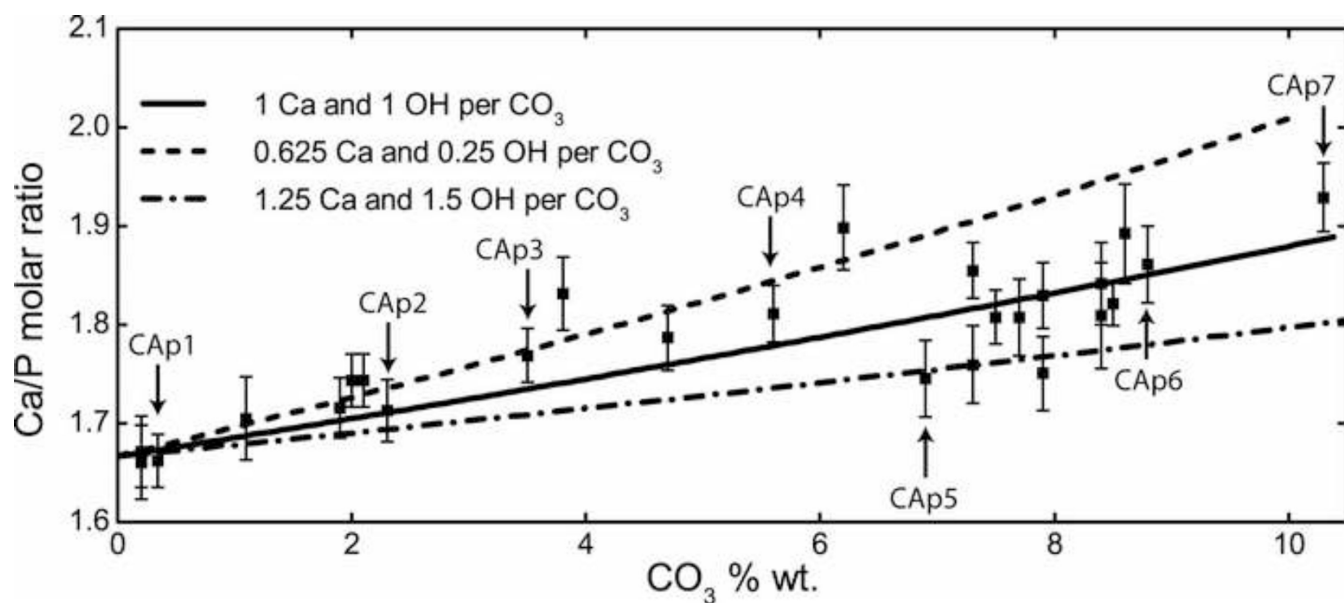
Figure 3. Plot of compositional analysis, Ca/P molar ratio of 26 B-type carbonated apatites versus \text{CO}_3^{2-} wt%. Modeled curves for high-ion loss (1.25 Ca and 1.5 OH per \text{CO}_3 ), medium-ion loss (1 Ca and 1 OH per \text{CO}_3 ) and low-ion loss (0.625 Ca and 0.25 OH per \text{CO}_3 ) are overlaid representing a variety of possible charge-balance mechanisms. Y-error bars represent standard deviations. Labeled CAP samples are characterized in Table 1.
