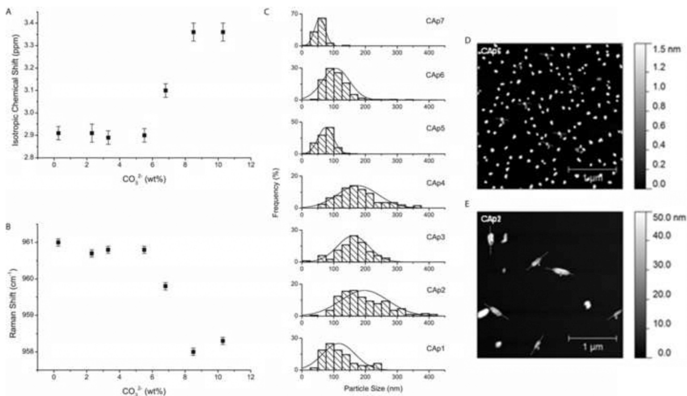
Figure 2. Characterization of carbonate-induced transition in synthetic carbonated apatites in the 0.3–10.3 wt% range. A) Measures of ^{31}\text{P} NMR chemical shift relative to \text{H}_3\text{PO}_4 , and B) Raman \text{PO}_4^{3-} band center versus carbonate content with error bars representing standard deviations. C) Histograms of carbonated apatite particle size distribution as measured by atomic force microscopy (AFM), with D) & E) micrographs of CAp6 (8.72 wt% \text{CO}_3^{2-} ) and CAp2 (2.26 wt% \text{CO}_3^{2-} ), respectively.
