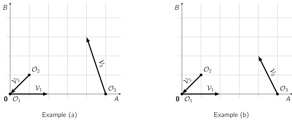
Figure 1. Two DRNs with 3 reactions involving 2 species A and B .
