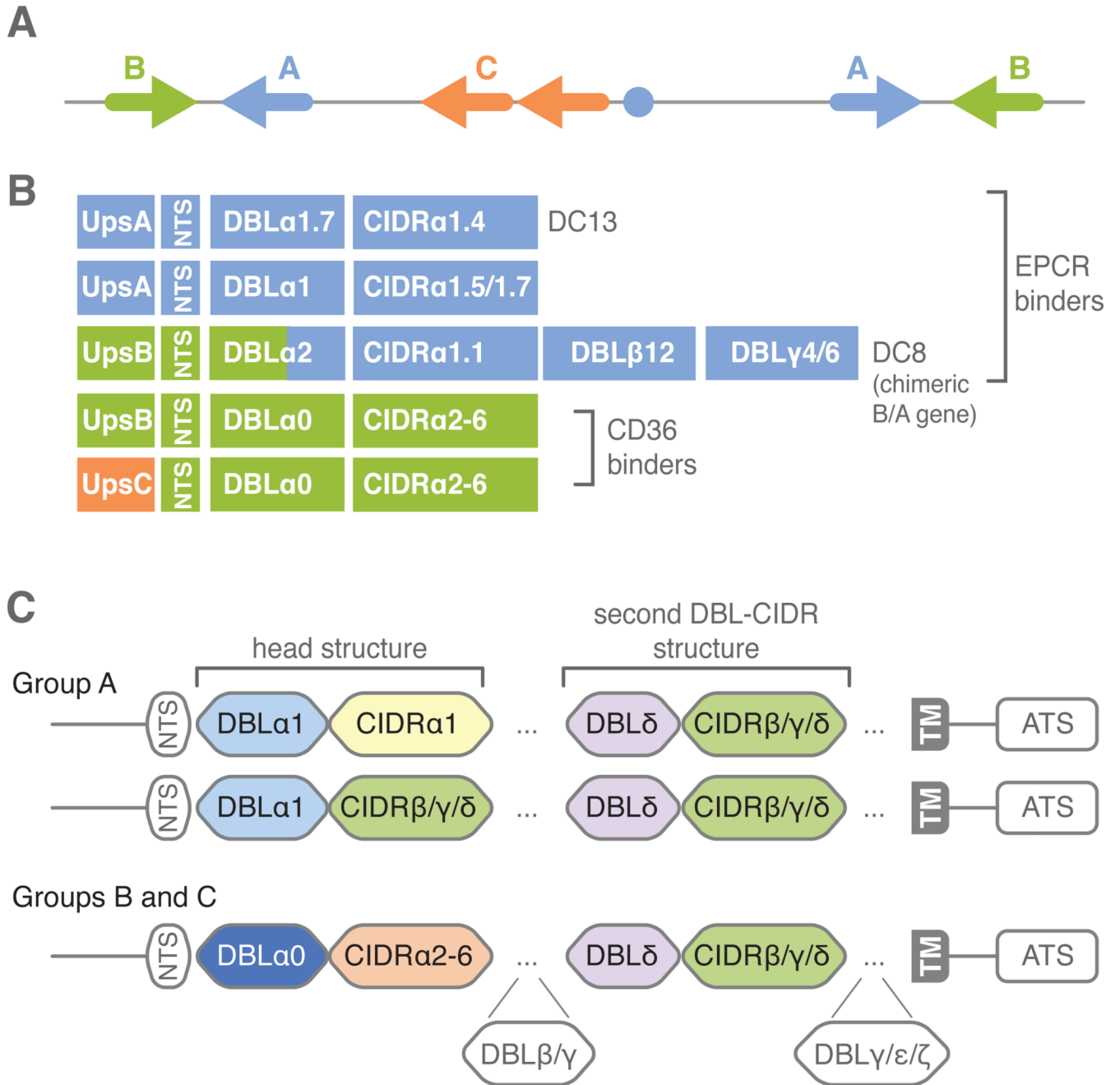
Fig. 1. Var gene organization and protein domain architectures. A. Chromosomal organization of var genes. Group B and A var genes are located in the subtelomeric regions and transcribed in opposite orientations. Group C are typically found on central chromosome clusters. B. There is a recombination hot spot between subdomains 2 and 3 in the DBL domain of the PfEMP1 head structure. DC8 is an unusual chimeric gene between a group B and group A var gene. C. Different types of DBL and CIDR domains are located at the N- and C-terminus of proteins. Small PfEMP1 have four extracellular domains, large PfEMP1 have additional DBL domains after the head structure or the second DBL-CIDR structure.
