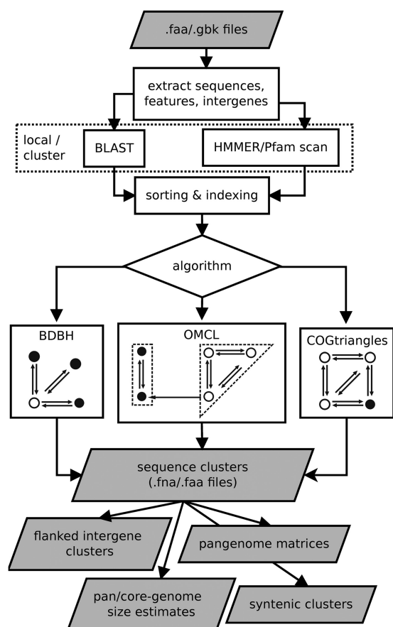
FIG 1 GET_HOMOLOGUES flow chart and its outcomes. BLAST and optional Pfam searches are optimized for local (multicore) and cluster computer environments. While the BDBH algorithm uses one sequence from the reference genome to grow clusters, the COG algorithm requires a triangle of reciprocal hits. Instead, the OMCL algorithm groups nodes in a BLAST graph to build clusters. Note that these clustering algorithms can be fine-tuned by customizing parameters such as -C (minimum percentage of coverage in pairwise BLAST alignments), -E (maximum E value for a hit to be considered), -D (require equal Pfam domain composition when defining similarity-based orthology composition), -S (minimum percentage of sequence identity in BLAST query/subject pairs [BDBH/OMCL]) and -N (minimum BLAST neighborhood correlation [BDBH/OMCL]). In addition, the user can choose which genome should be used as the reference using option -r .
